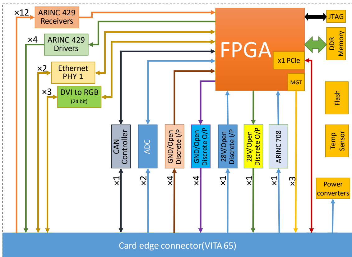
Figure 1: Interface Processing Card Block Diagram
