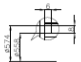
DETAIL-A (O-RING GROOVE)
