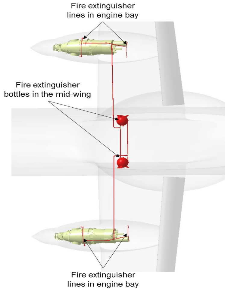
Figure 3: Engine Fire Extinguisher System Layout
