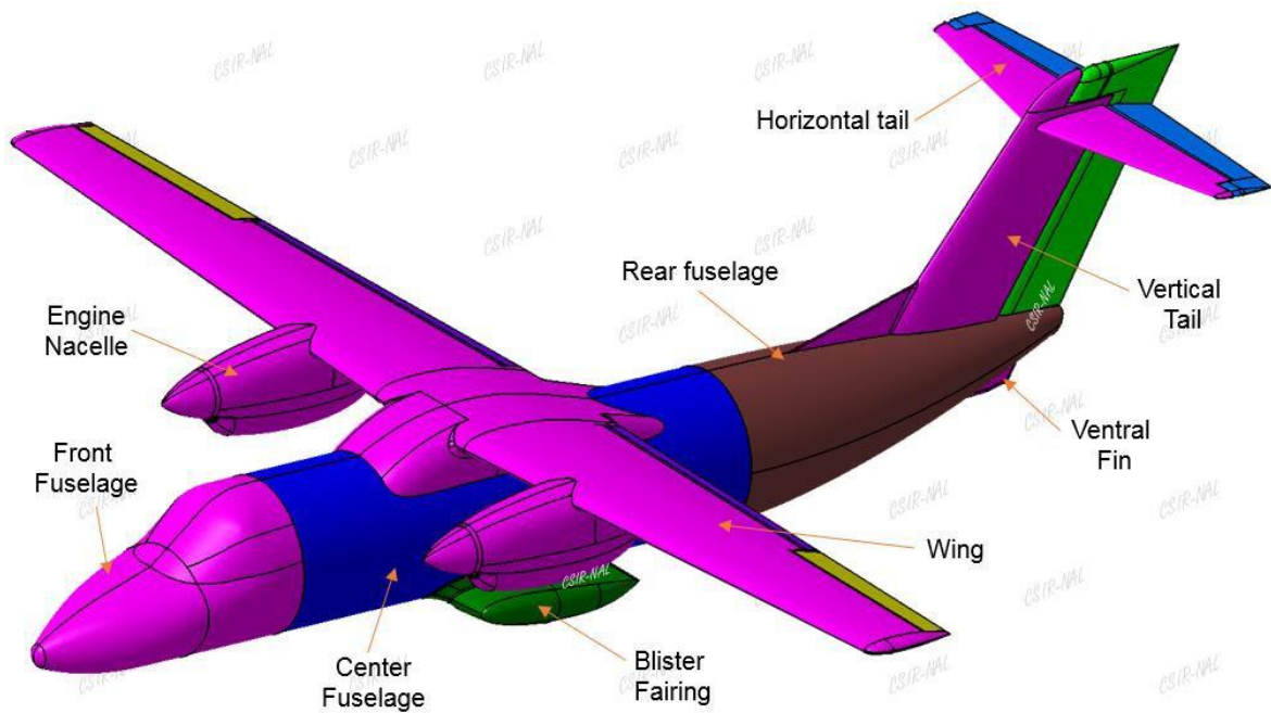
Figure 1: SARAS Mk2 configuration
