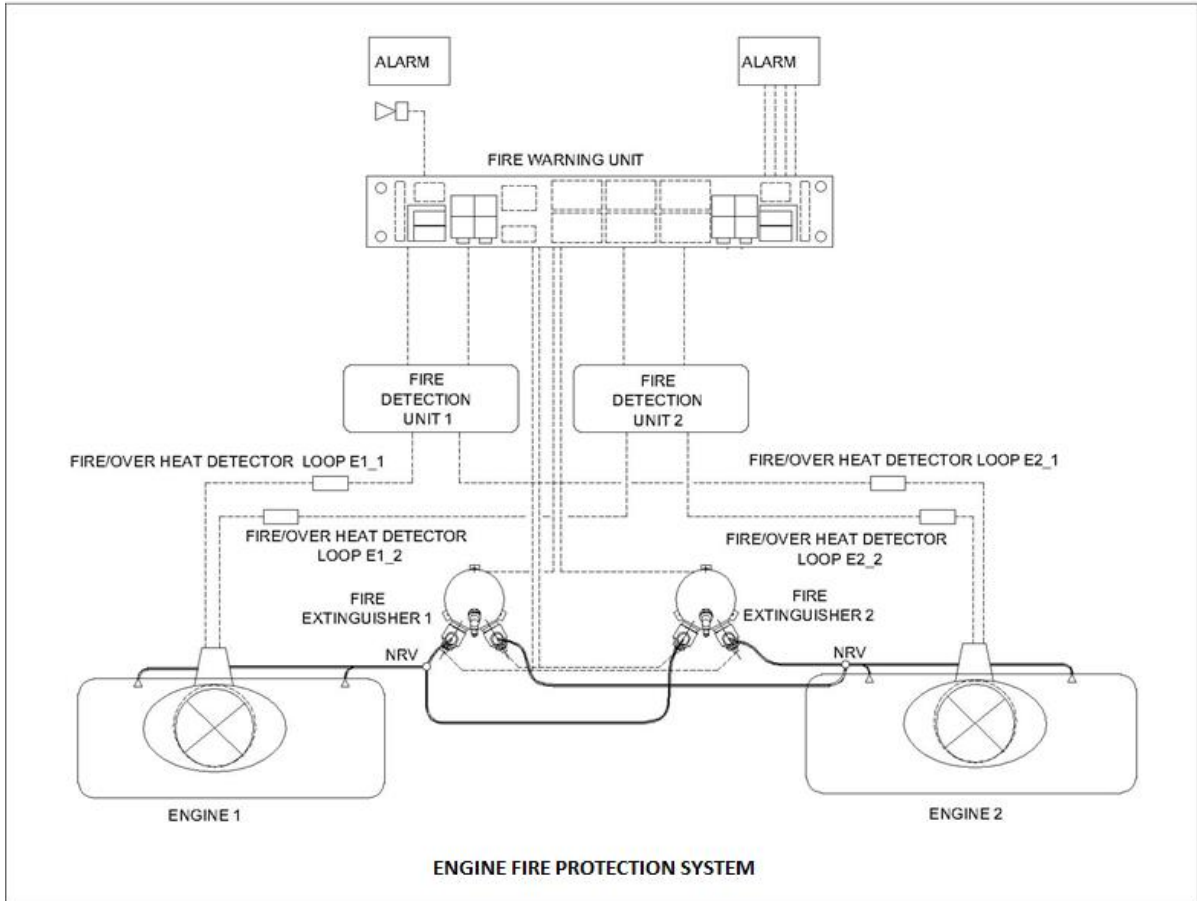
Figure 1: EFPS Architecture
