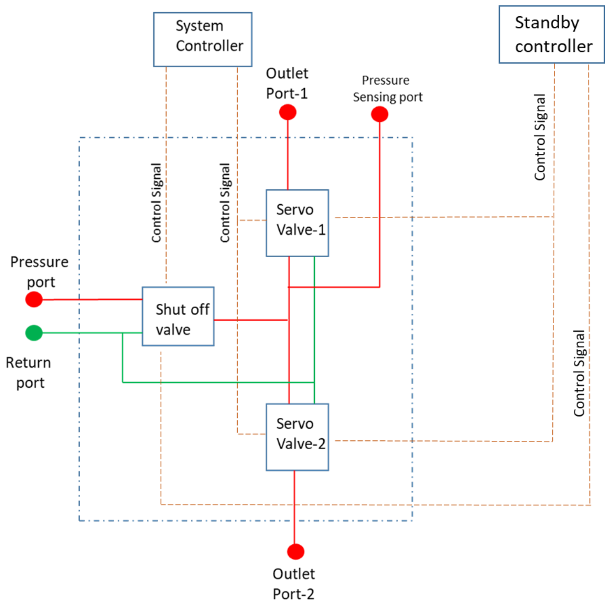
Figure 1: Typical Brake Manifold Architecture
