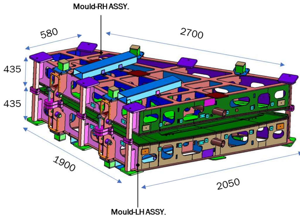
Fig.1: Mould Assembly (Assembly of LH and RH mould assemblies)
