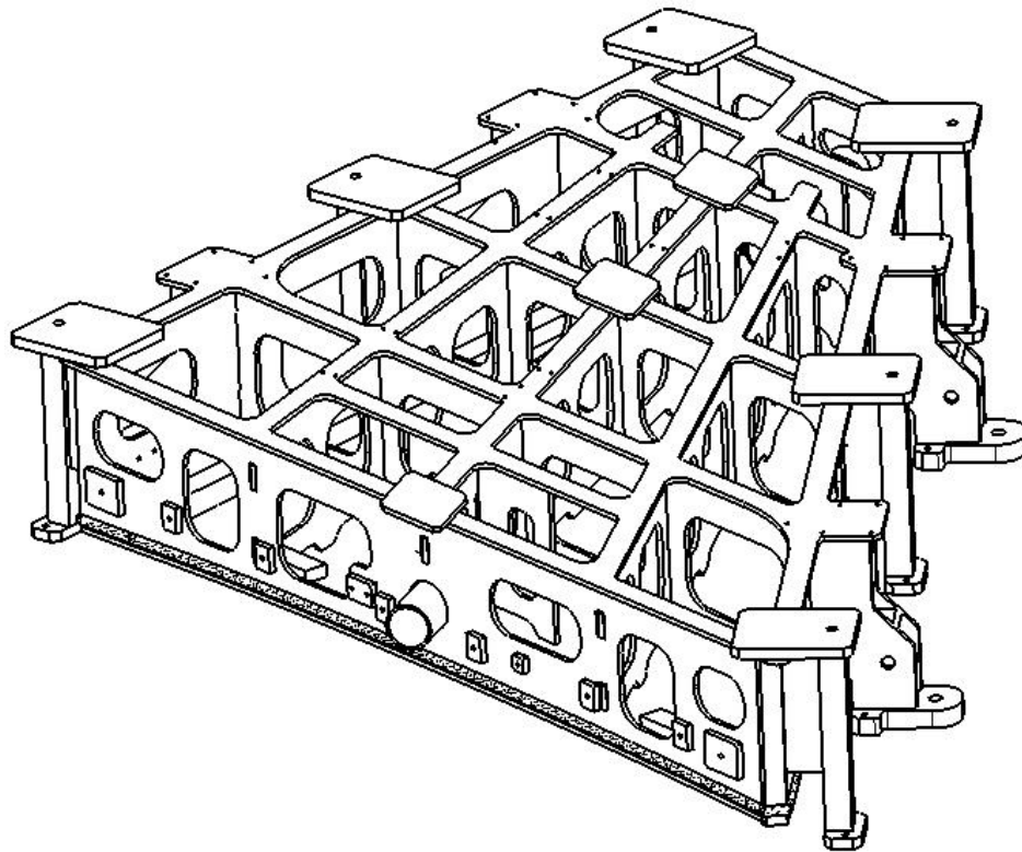
Fig.3: Mould-RH Assembly
