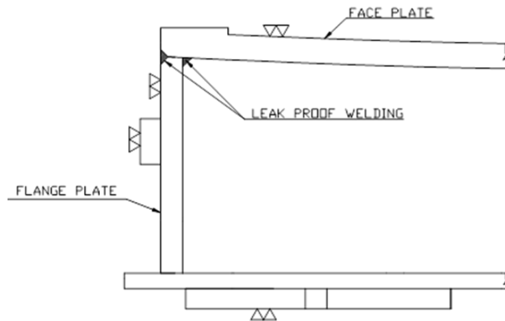
Fig.4: Typical leak proof welds between Faceplate and Flange plate
