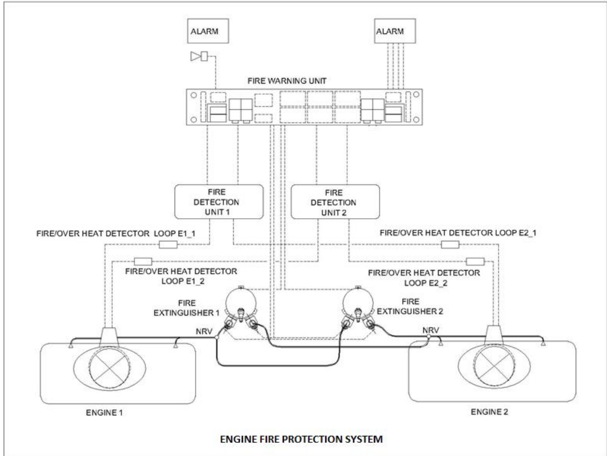
Figure 1: EFPS Architecture
