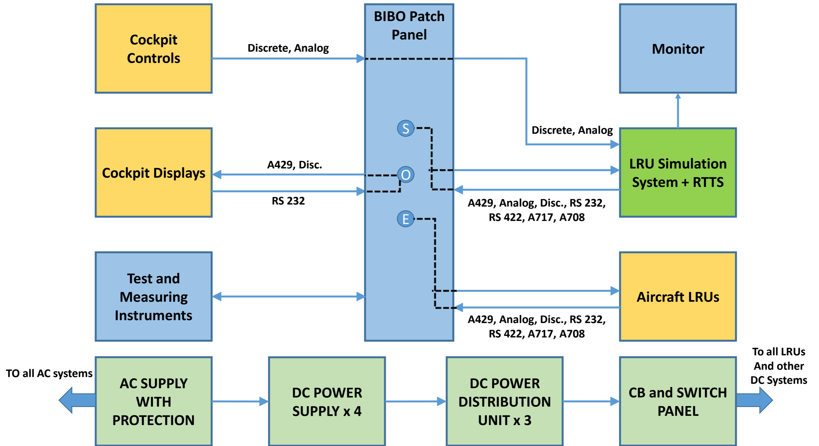
Figure 1: Overview of AITR
