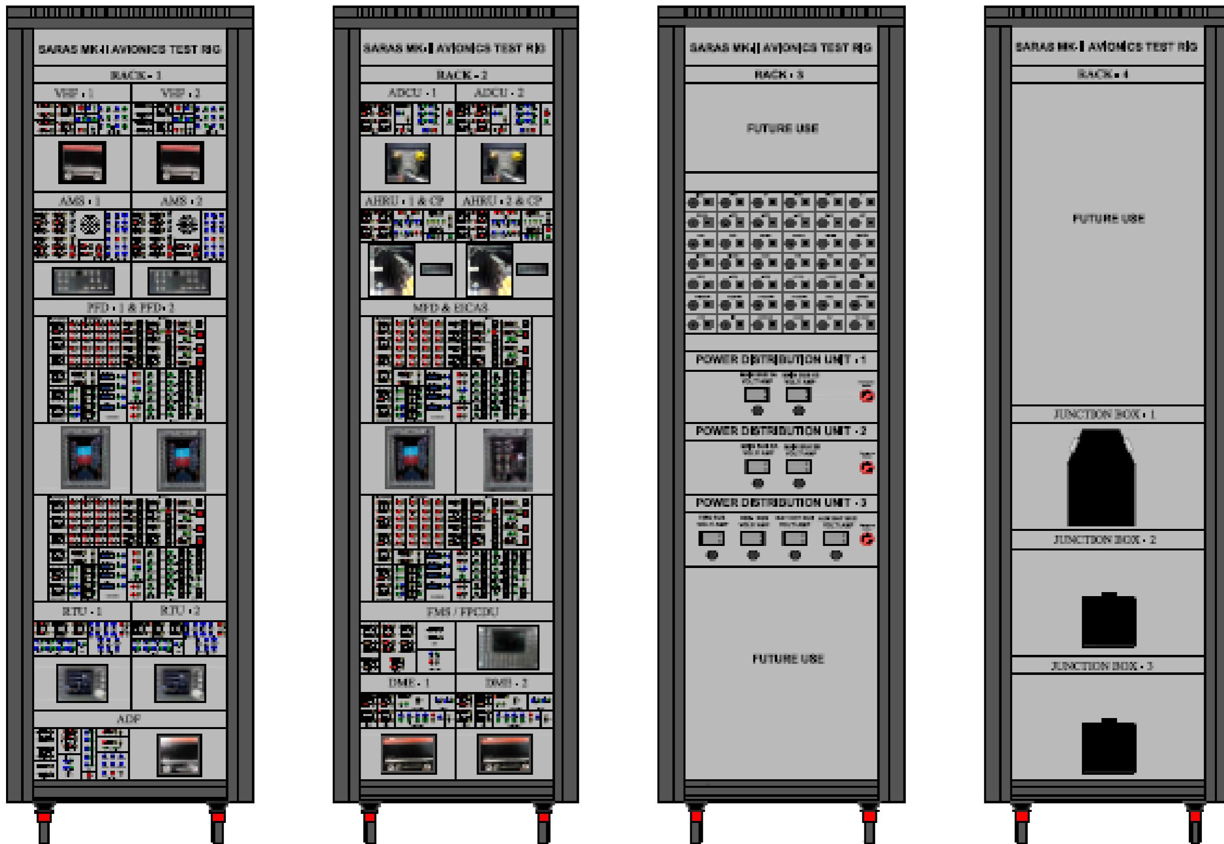
Figure 3: Arrangement of ATR Racks – 1
