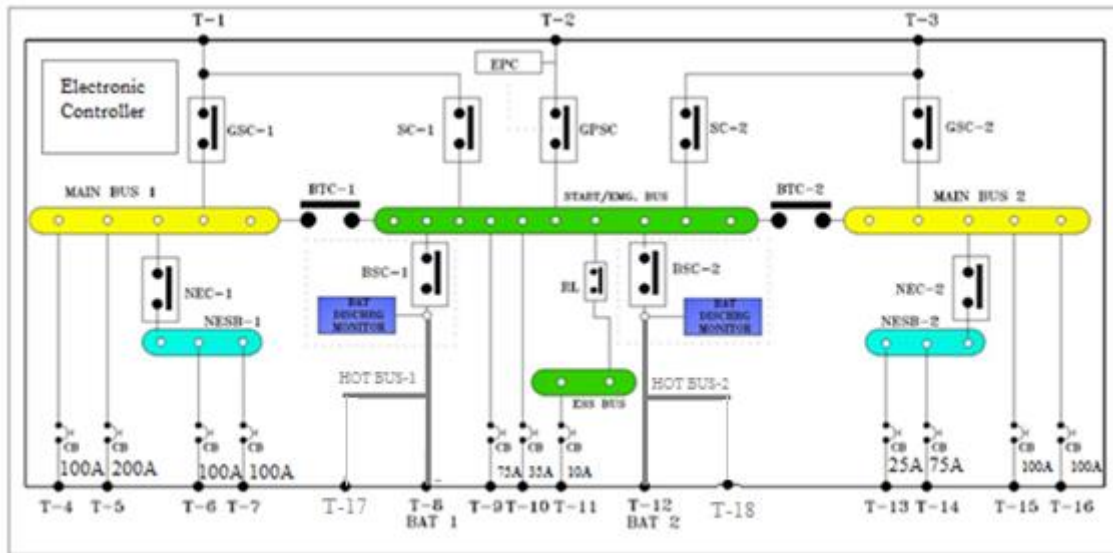
Figure 1: Typical Primary Power Distribution System Architecture
