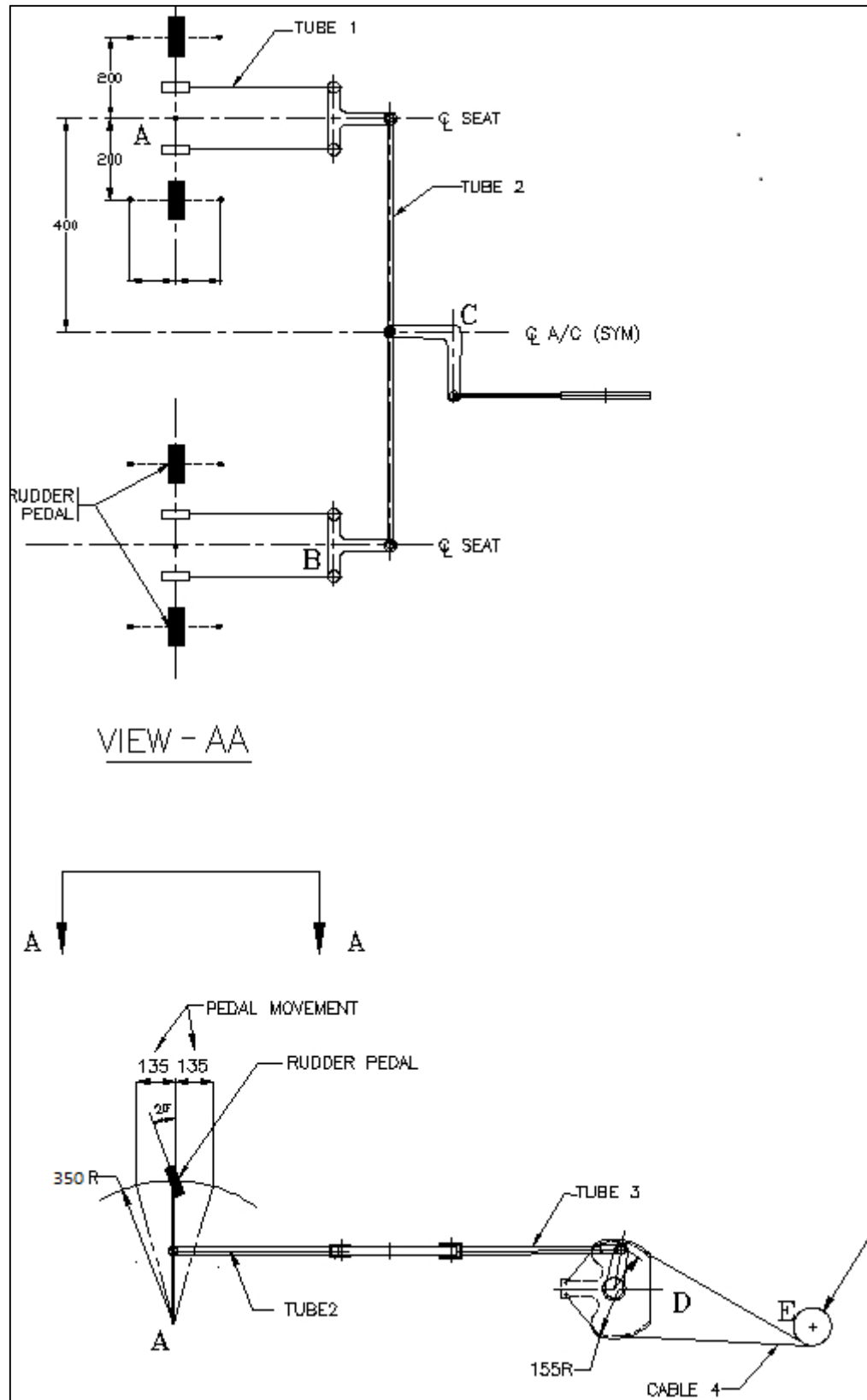
Figure 3 Rudder Control Circuit
