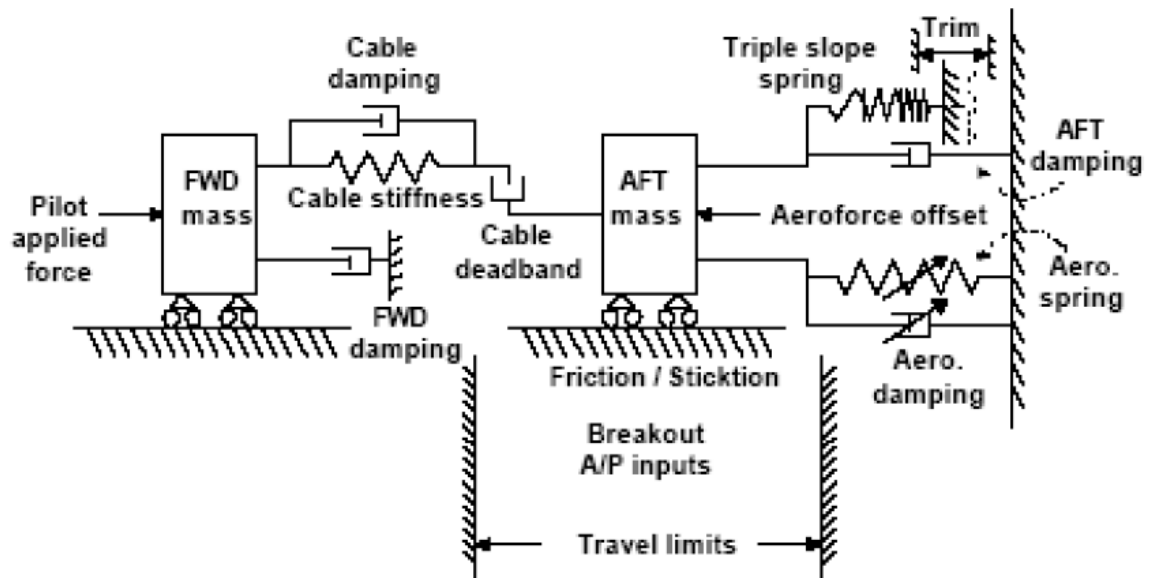
Figure 5. Equivalent Spring / Mass / Damper System of SARAS Mk2 mechanical PFCS
