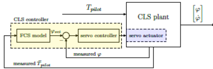
Figure 4. Schematic of proposed CLS
