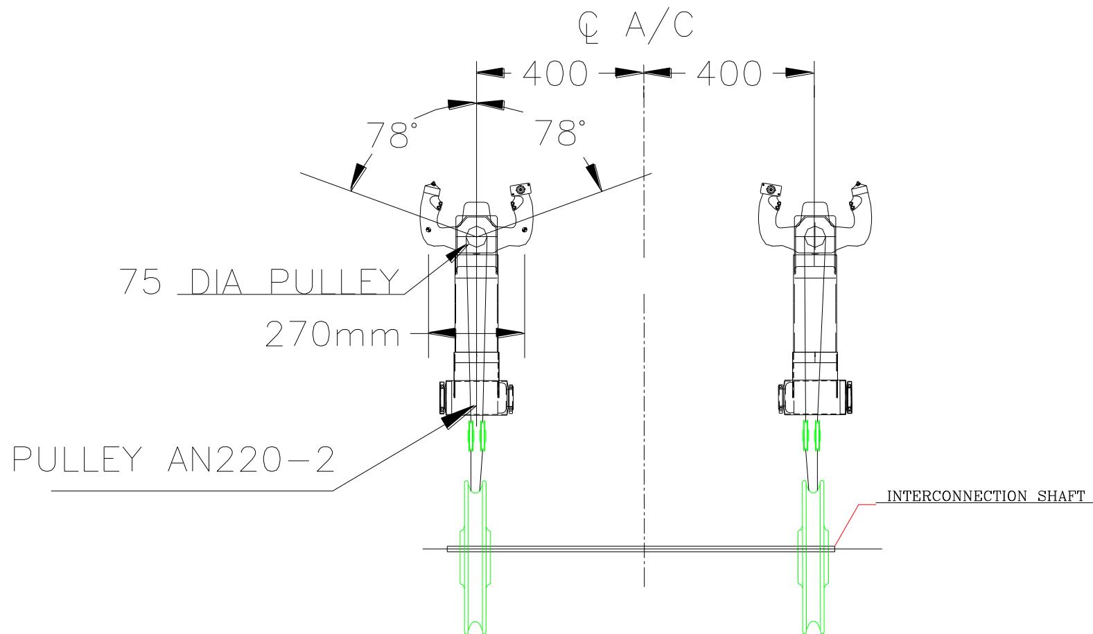
Figure 1 Aileron Control Circuit
