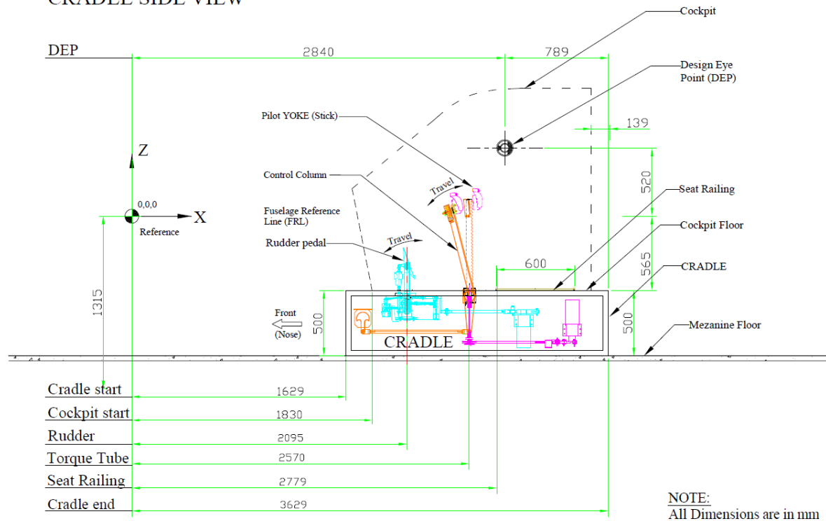
Figure 8. Side view of representative cradle
