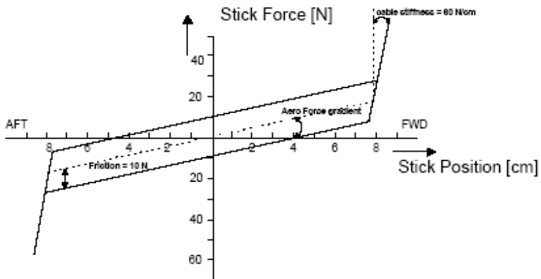
Figure 6. Airborne Control Feel of Manual Flight Control
