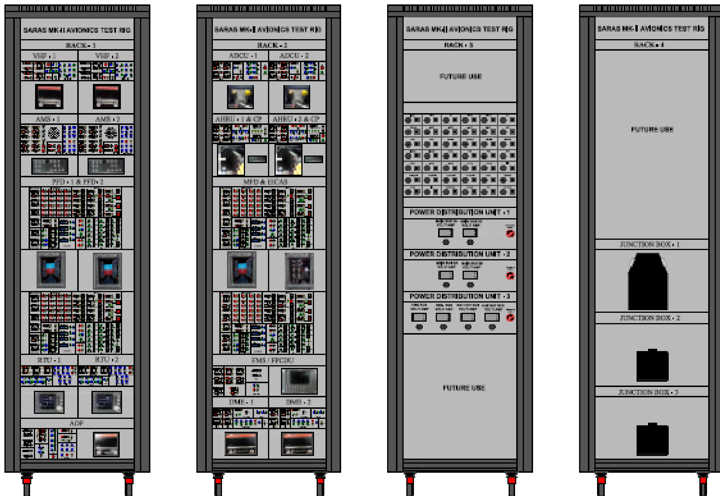
Figure 3: Arrangement of ATR Racks – 1
