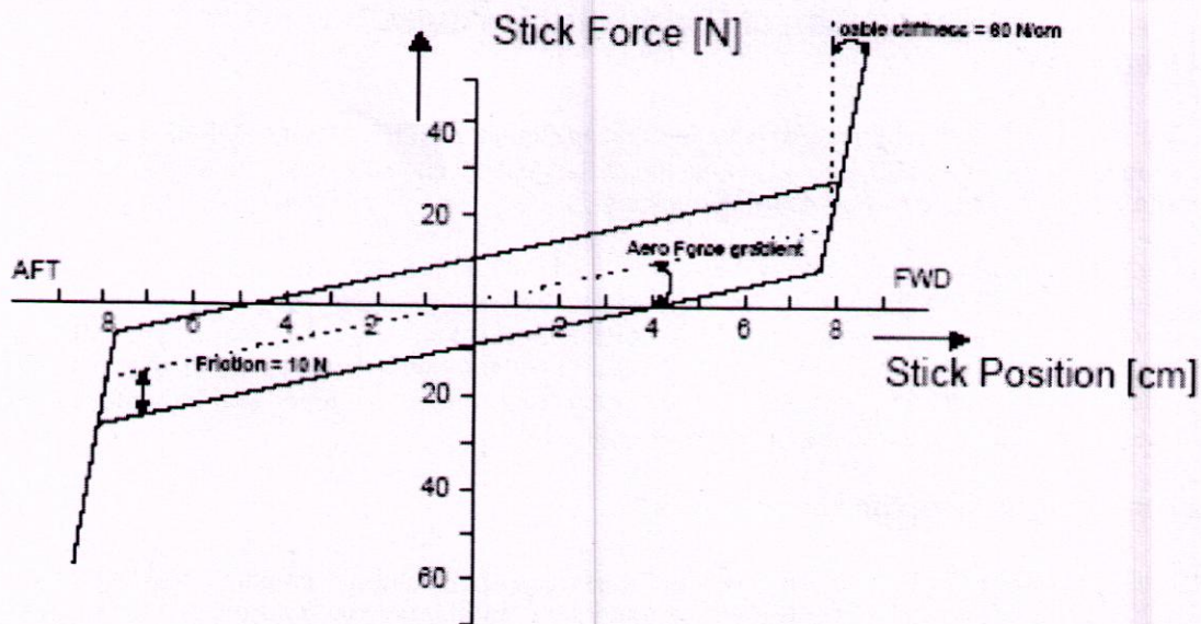
Figure 4.2.3.2. Airborne Control Feel of Manual Flight Control
