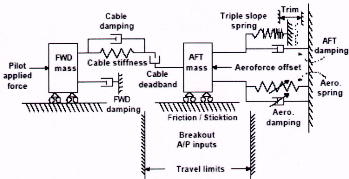
Figure 4.2.3.1. Equivalent Spring / Mass / Damper System of SARAS Mk2 mechanical PFCS
