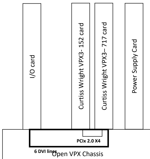
Figure 1 Architecture of Integrated Avionics Display Computer
