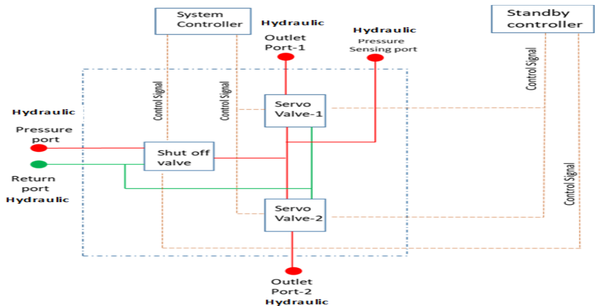
Figure 1: Required Brake Manifold Architecture
