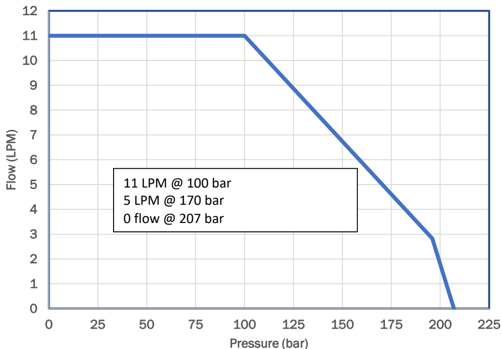
Fig 3: Required Pressure rise Vs Flow rate characteristics of Ground Hydraulic System
