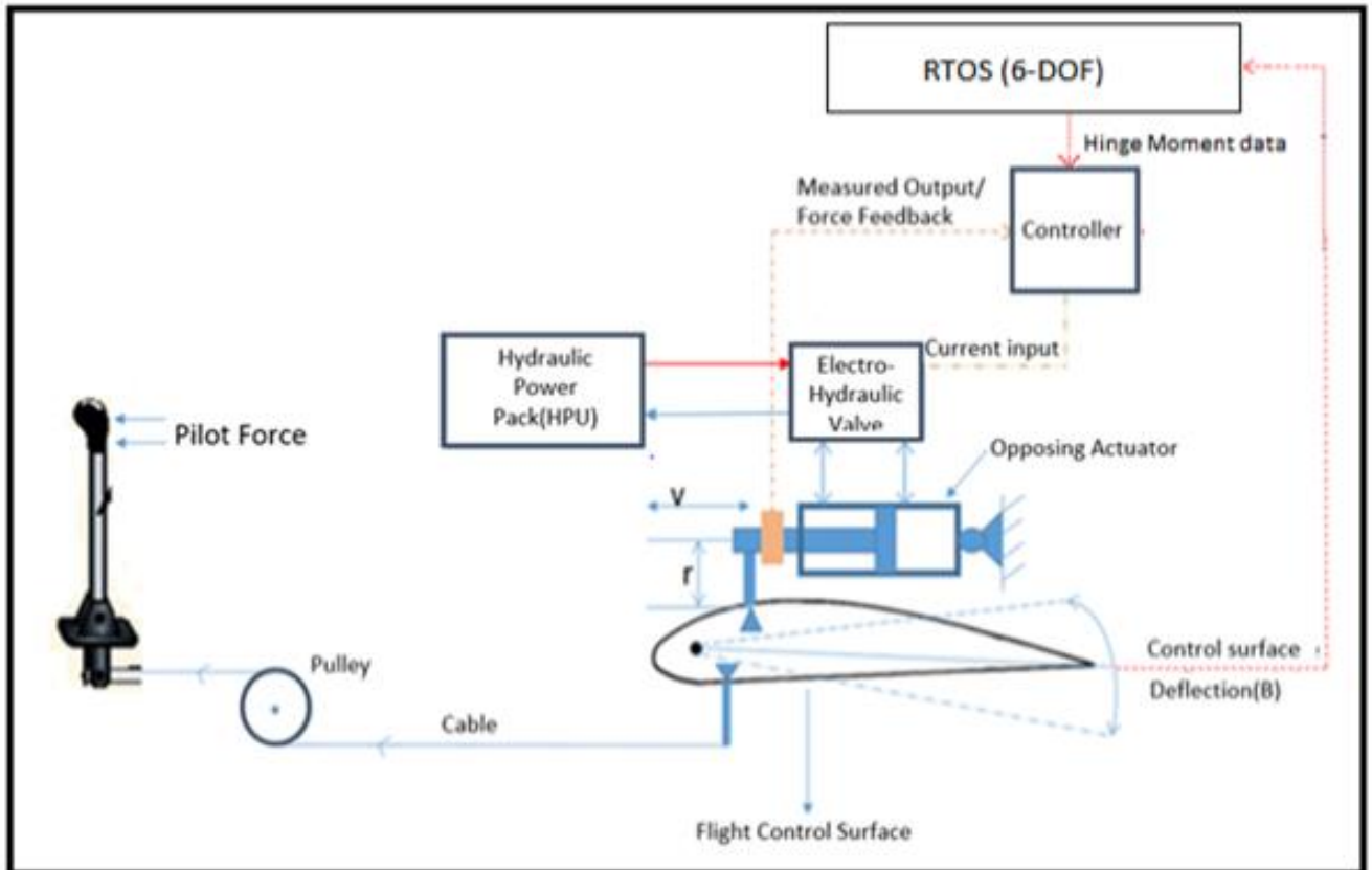
Figure 2: Proposed Control Loading System Architecture
