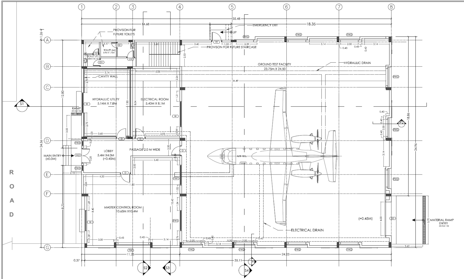
TYPICAL TESTING SITE LAYOUT FOR THE IRON-BIRD
