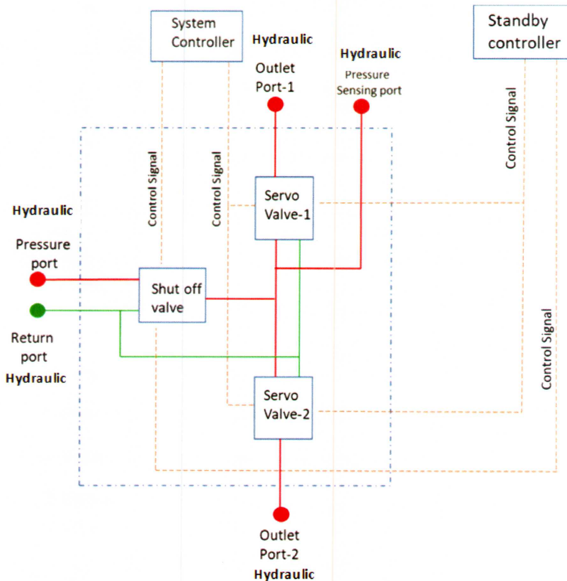
Figure 1: Required Brake Manifold Architecture
