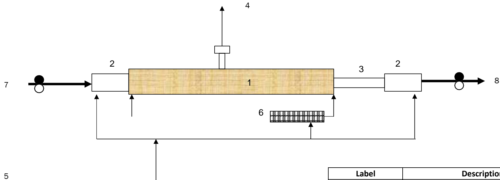
Annexure 2 Schematic representation of Low Temperature Furnace
