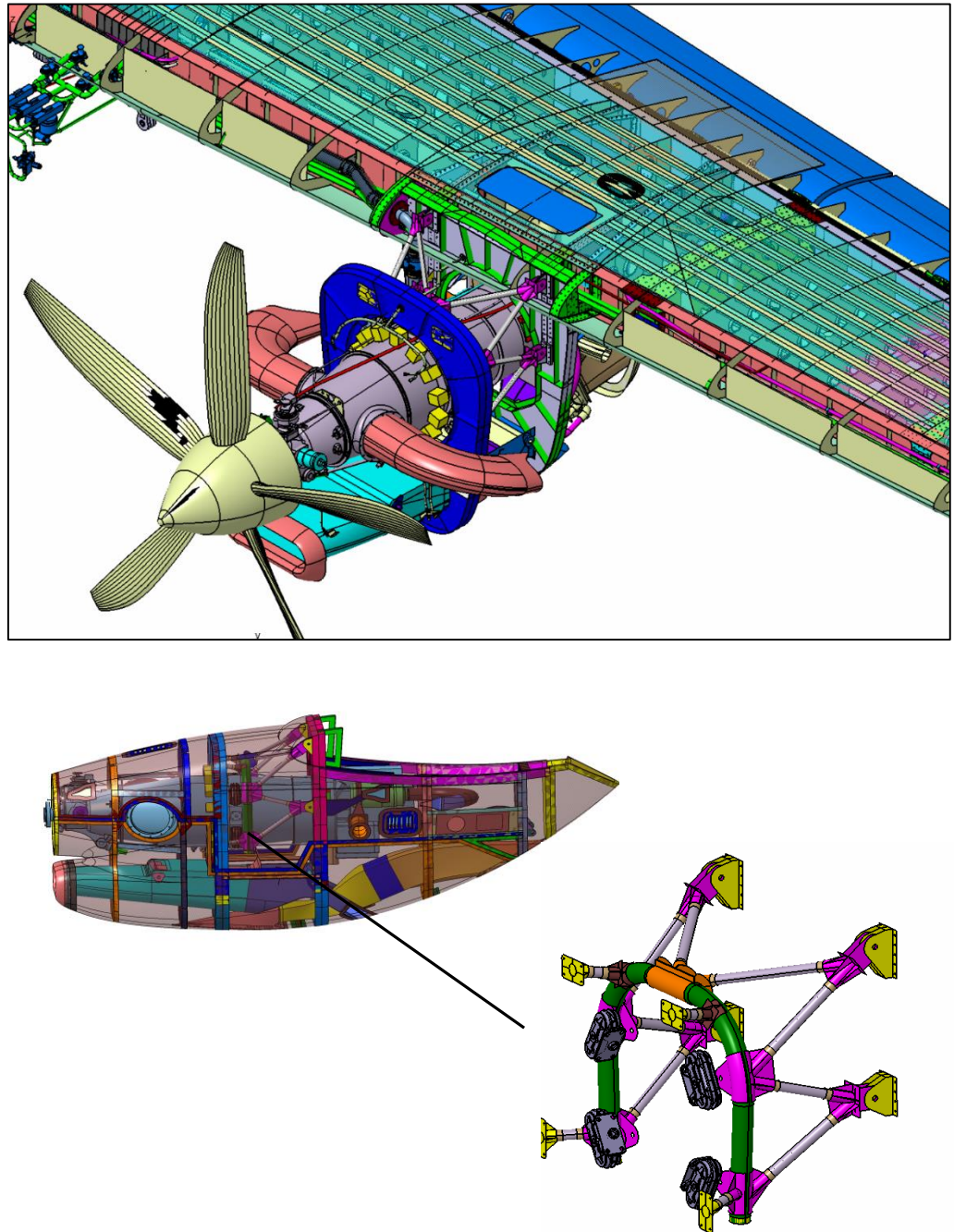
Fig 1.0 Engine Mount System
