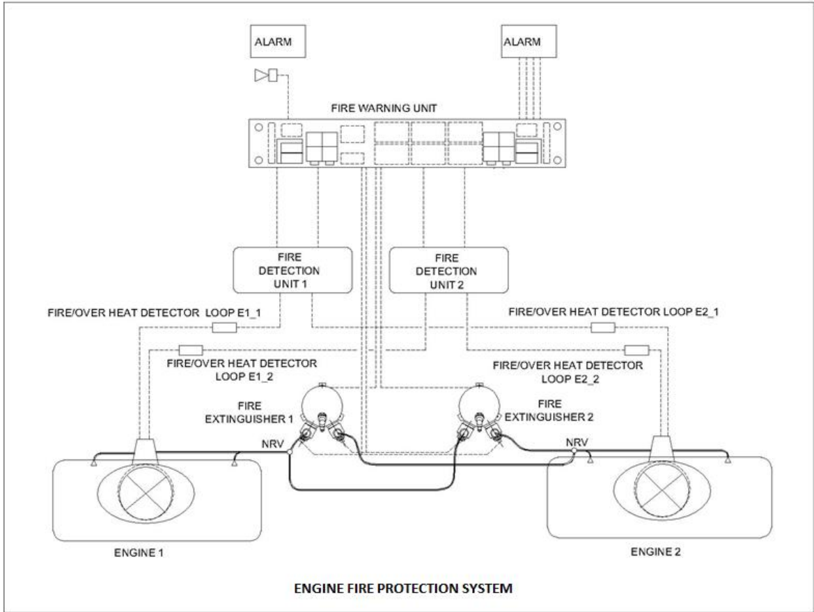
Figure 2: Typical Architecture of Engine Fire Detection System
