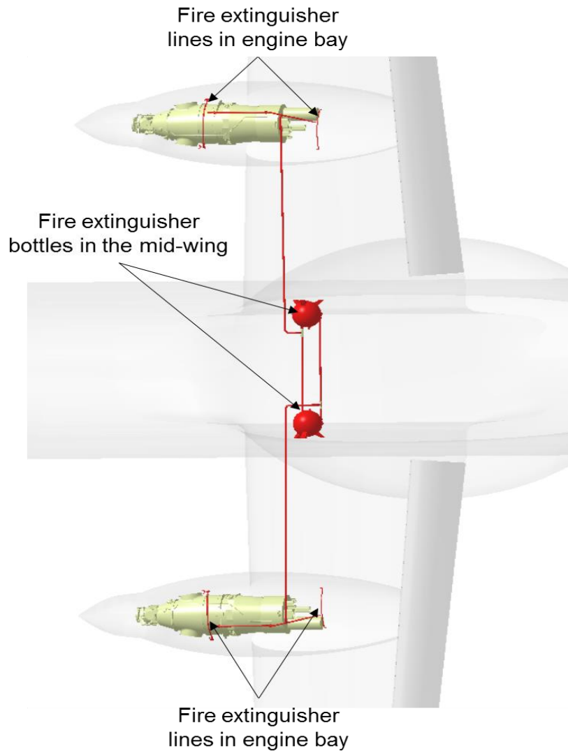
Figure 3: Engine Fire Extinguishing System Layout
