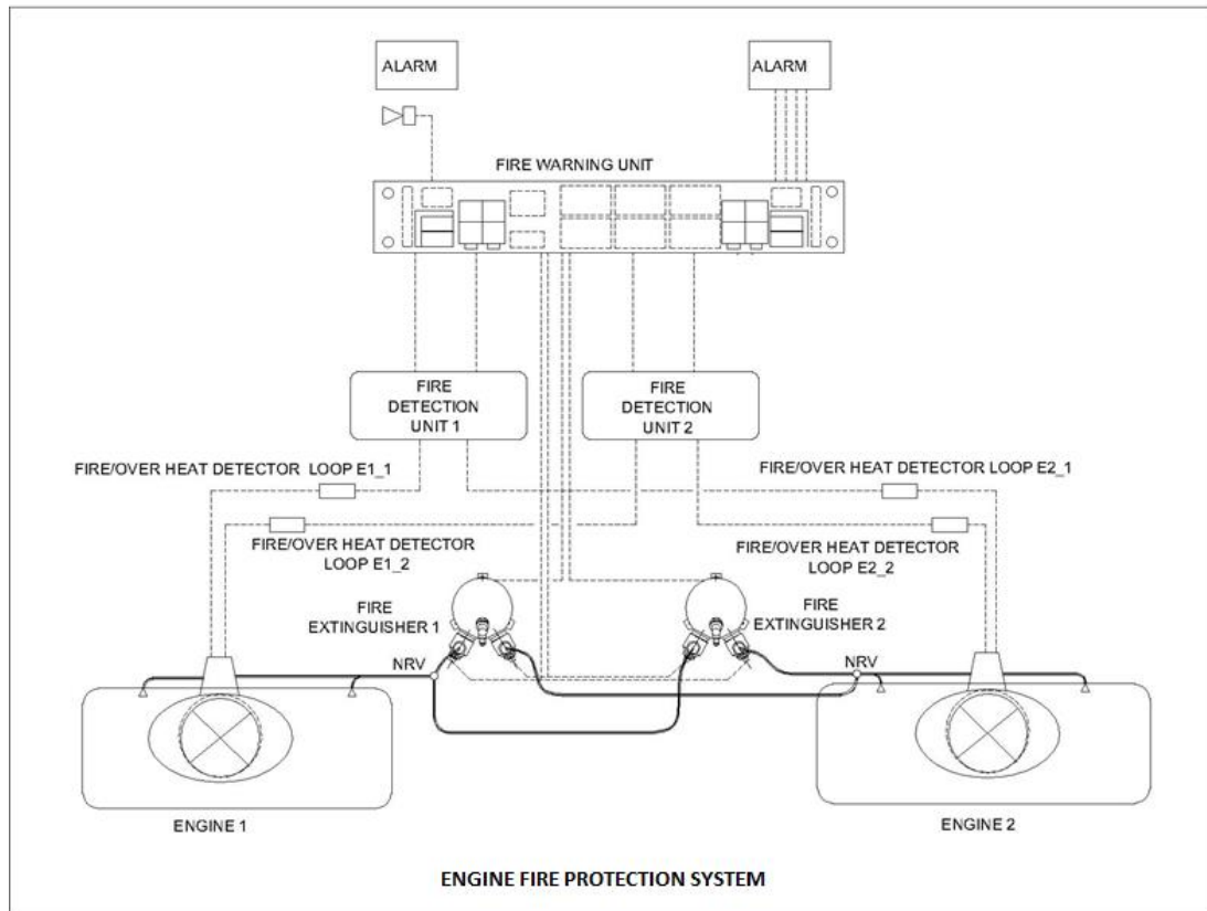
Figure 2: Typical Architecture of Engine Fire Detection System
