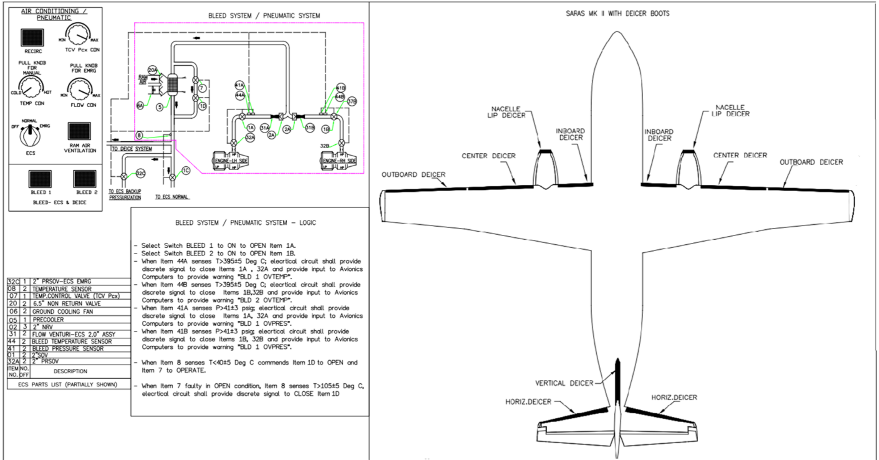
Figure 1 shows Saras Mk II Aircraft with Pneumatic Deicers. Bleed System/Pneumatic System is shown for reference. The Bidder shall propose suitable architecture based on off-the-shelf items as far as possible to meet the requirements of System specifications and safety, Reliability requirements as per FAR 23.1309 amendment 23-64. Ice detectors location shall be identified by the Bidder.
