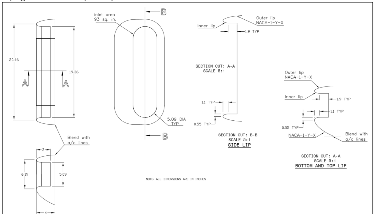
Figure 2: Saras Mk II Aircraft - Engine Air Intake Lip
