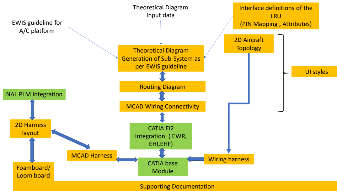
Figure1 : EWIS 2D design tool flow and 3D CATIA integration requirement of NAL
