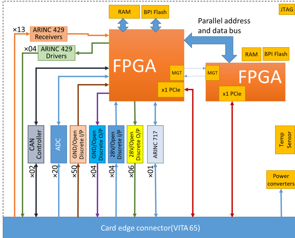
Figure 1 Block diagram of IOM
