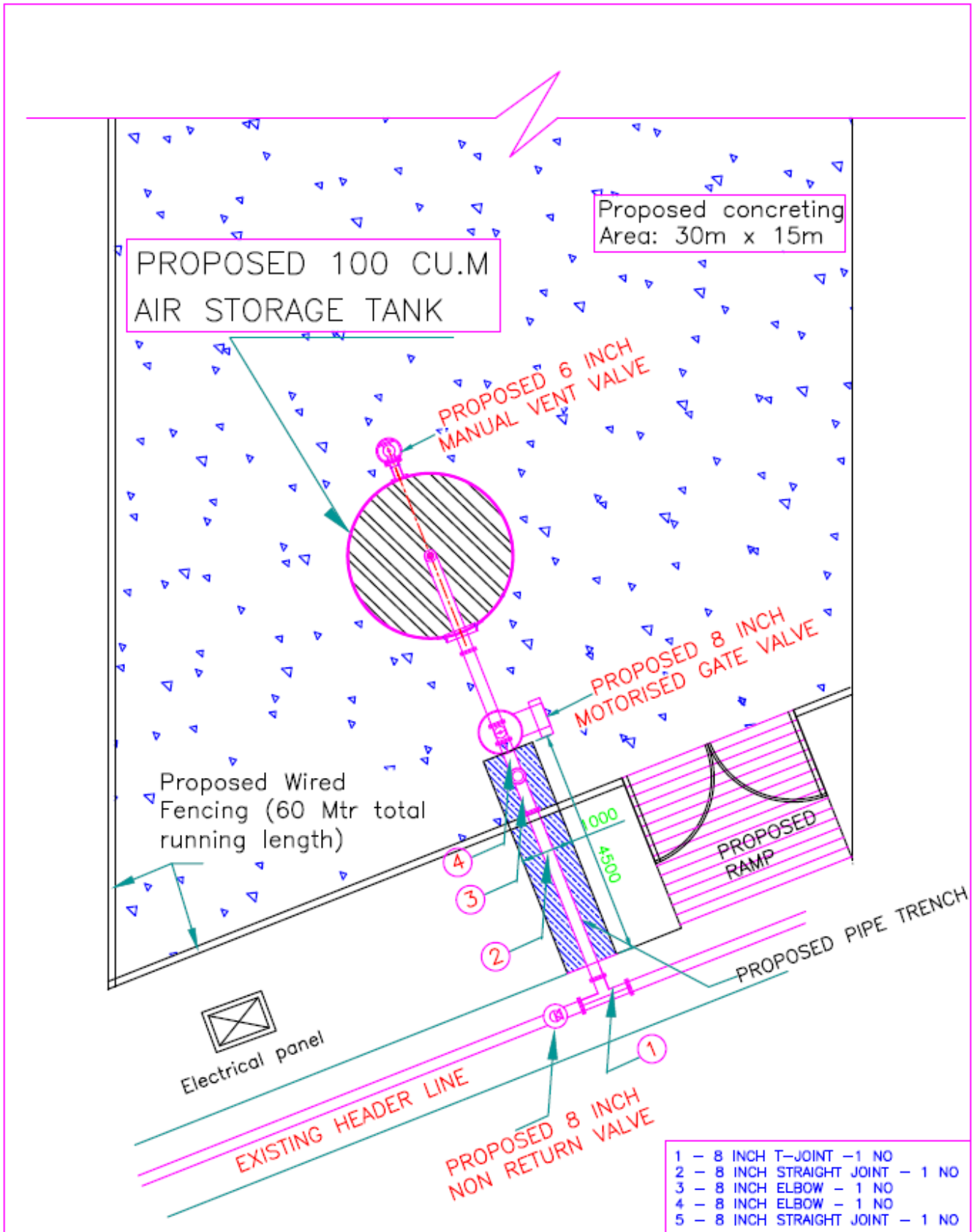
AIR STORAGE TANK PIPING, VALVES & TRENCH LAYOUT DETAILS
