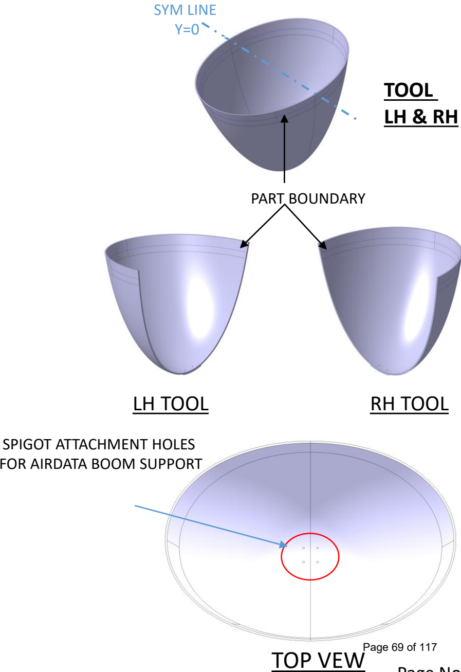
Fig. 03. TOOL FACE SHEET DETAILS
