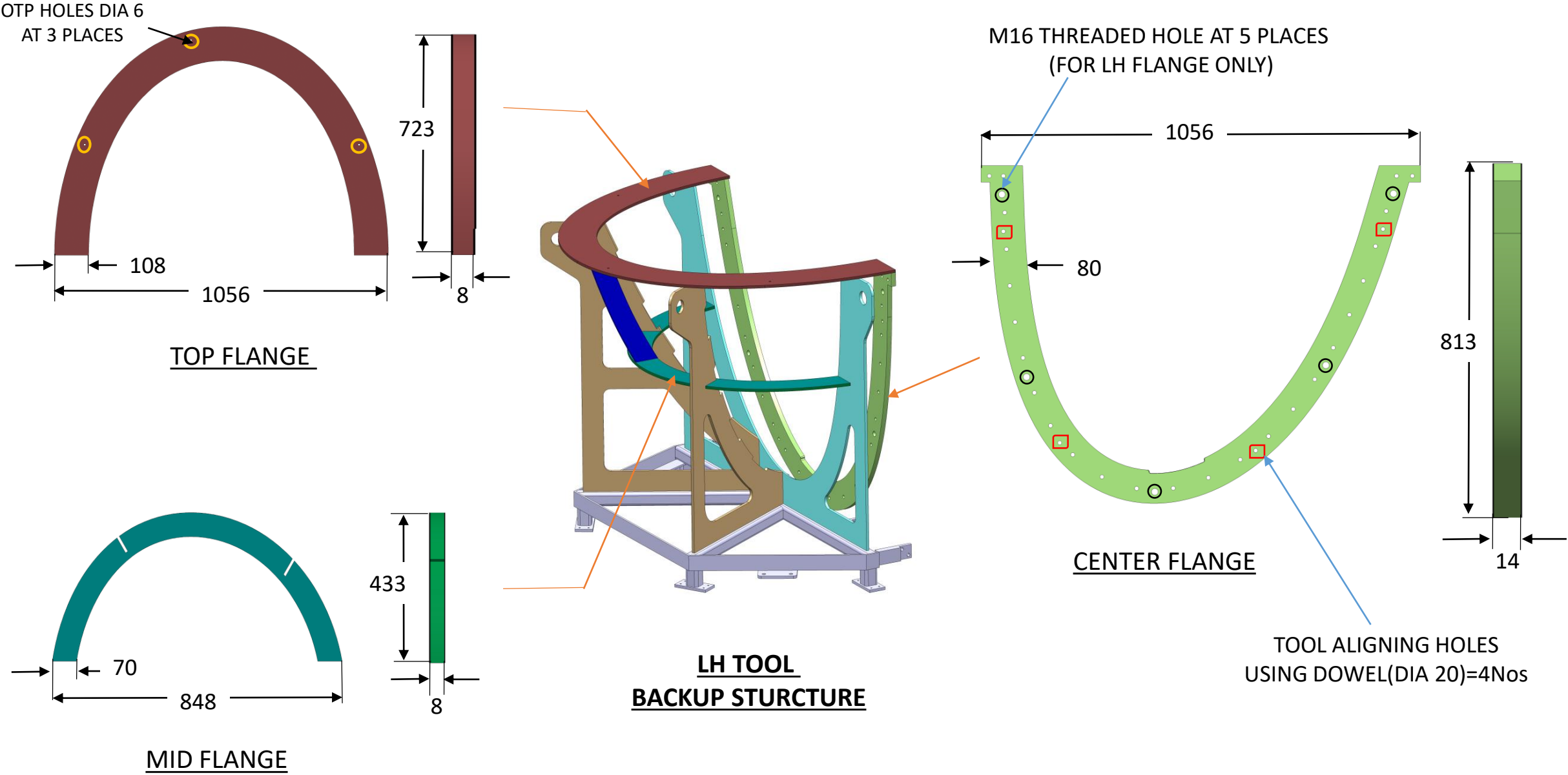
Fig. 07. LH TOOL FLANGE DETAILS
