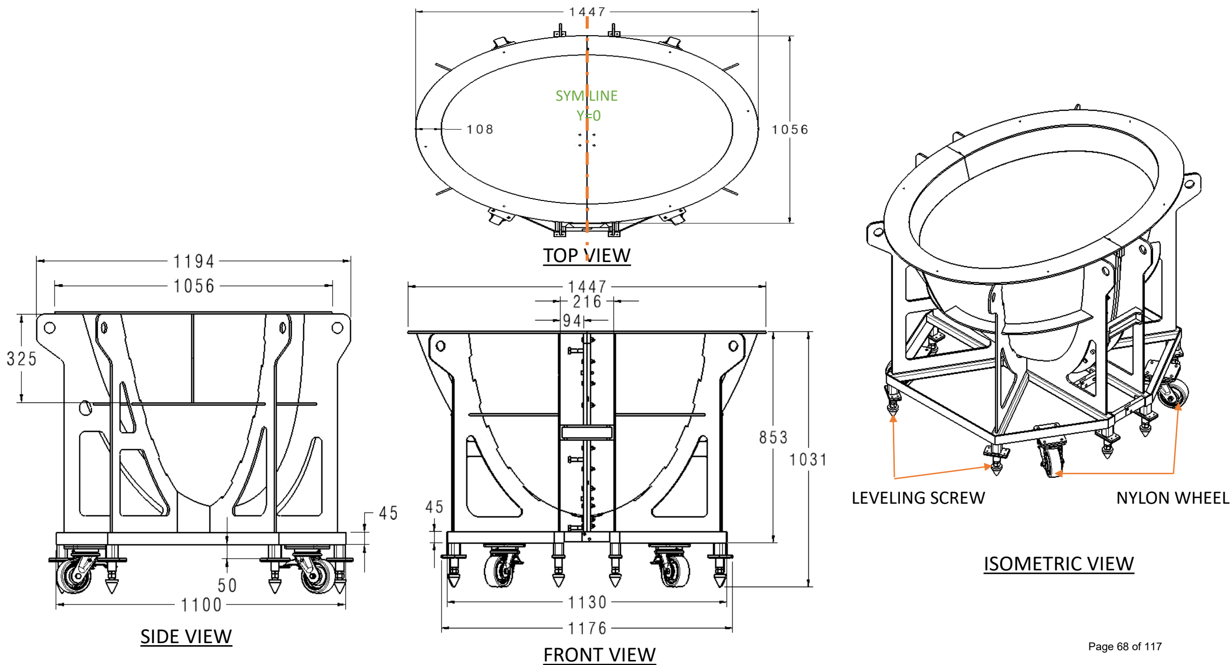
Fig. 01. TOOL FOR RADOME NOSE CONE (Schematic diagram)
