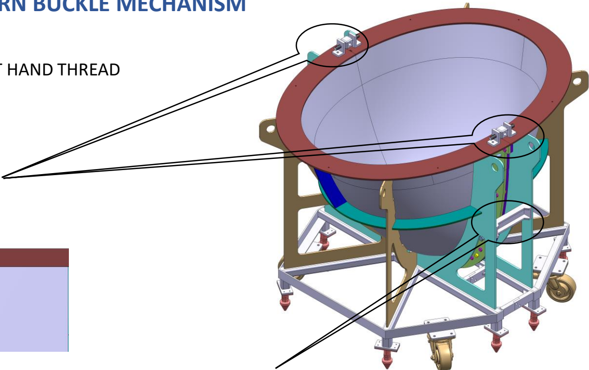
Fig. 10.TURN BUCKLE MECHANISM
