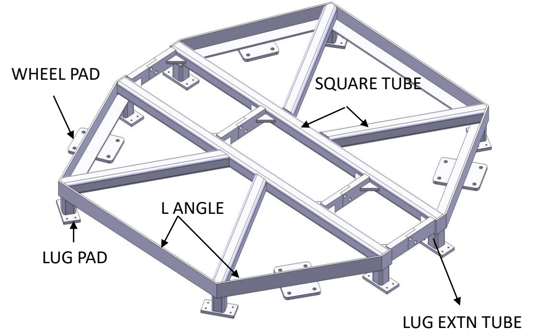
ISOMETRIC VIEW LH & RH MOULD BASE
