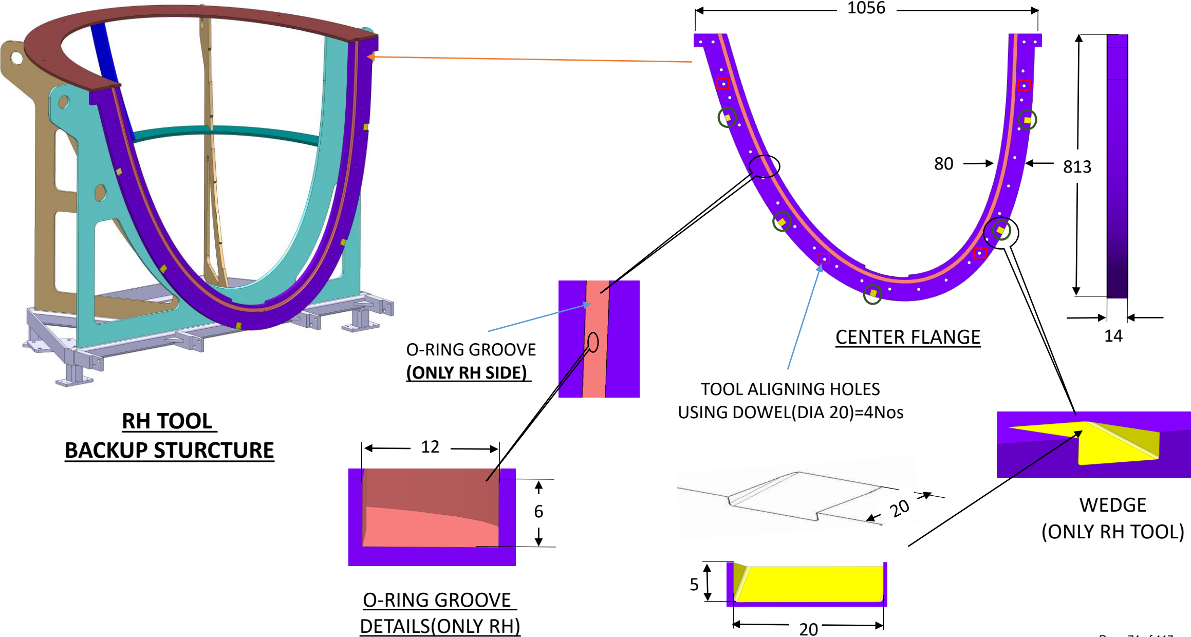
Fig. 08. RH TOOL FLANGE DETAILS
