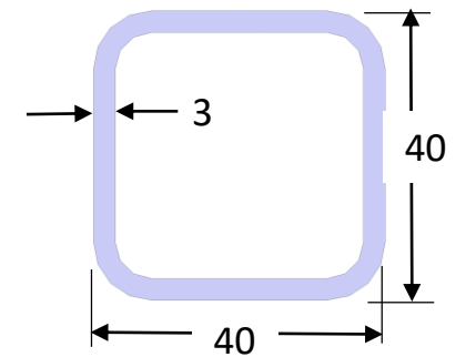
SQUARE TUBE DETAILS
