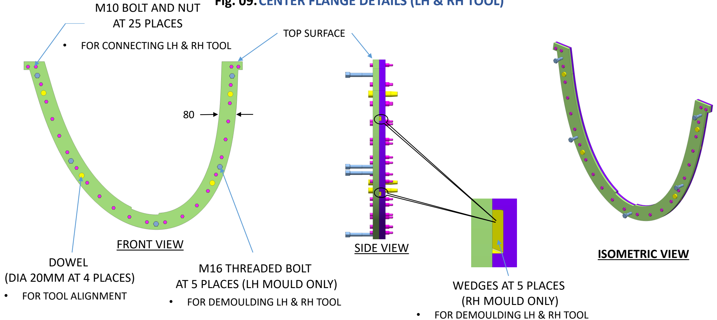
Fig. 09. CENTER FLANGE DETAILS (LH & RH TOOL)
