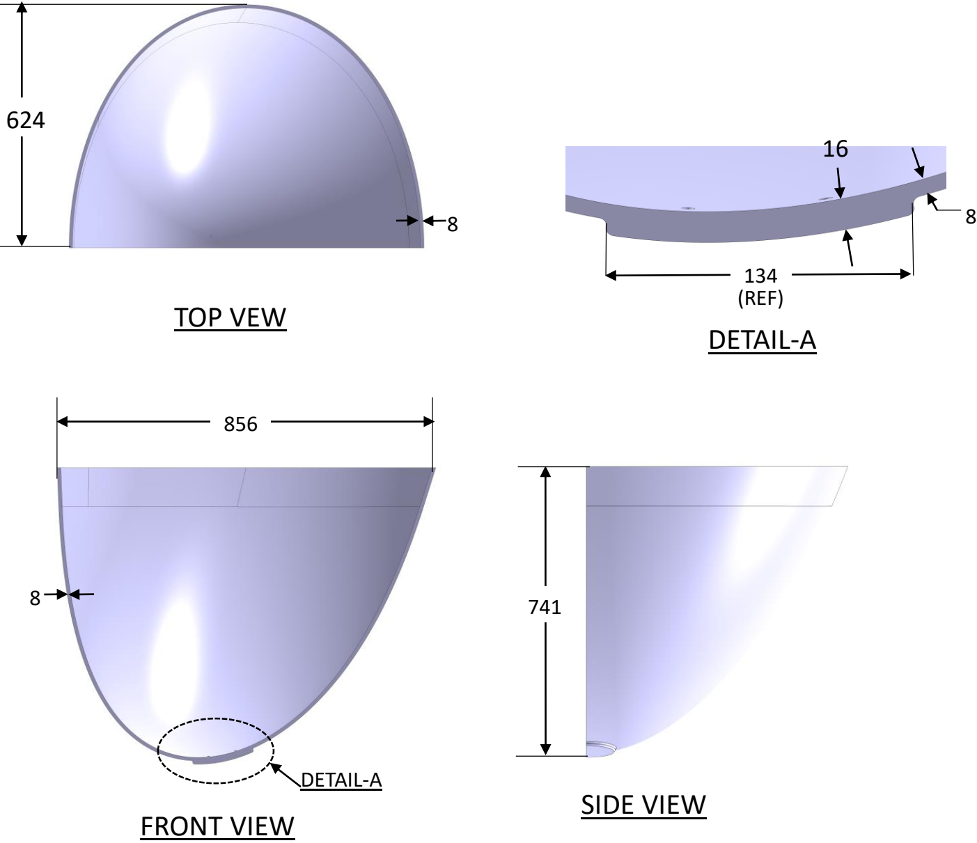
Fig. 02. LH TOOL FACE SHEET DETAILS
