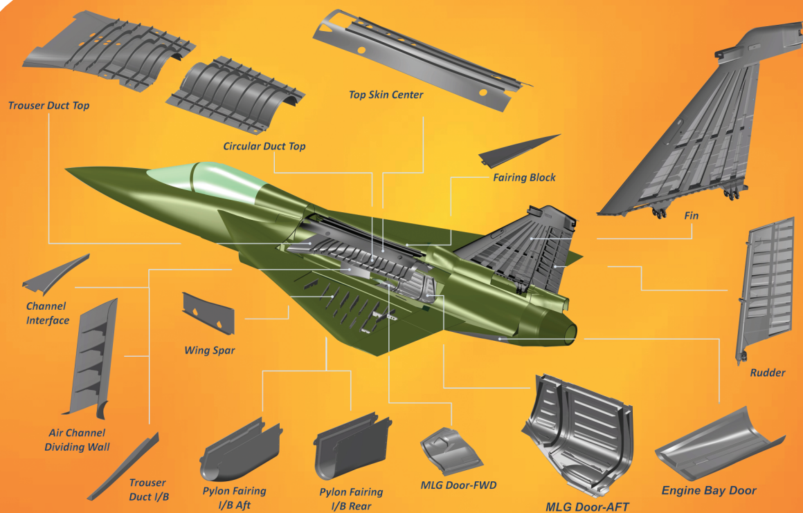
CSIR-NAL's Role in Light Combat Aircraft LCA-Tejas Airframe
