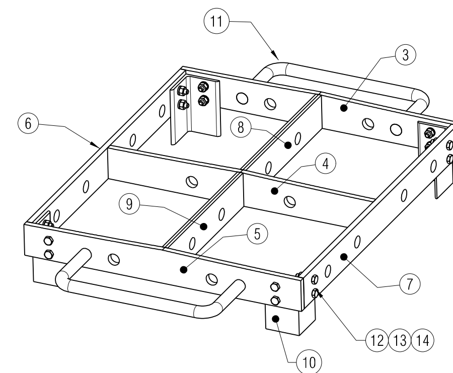
ISOMETRIC VIEW SCALE: NTS (BACKUP STRUCTURE)
