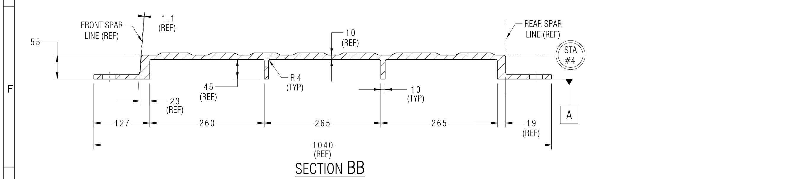
DETAIL OF ITEM No.1 (CAUL PLATE MASTER)
