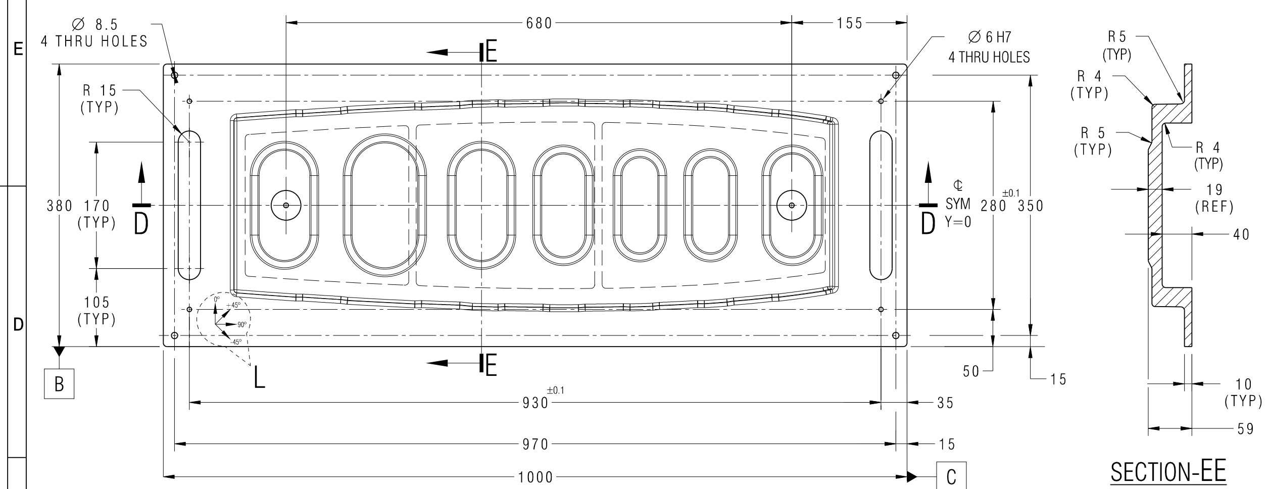
DETAIL OF ITEM NO:1 (CAUL PLATE MASTER)
