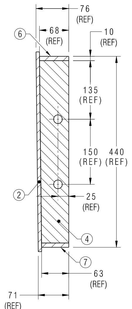
SECTION GG
