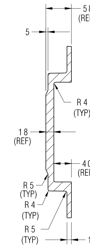
SECTION FF
