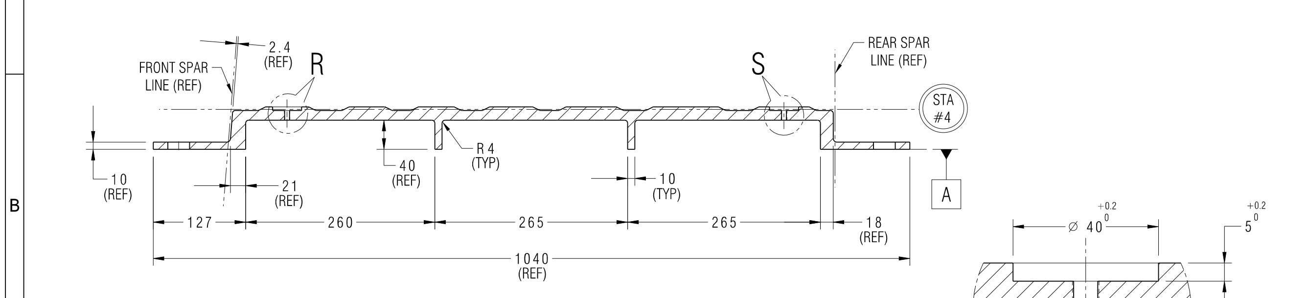
DETAIL OF ITEM No.2 (LAYUP CORE)
