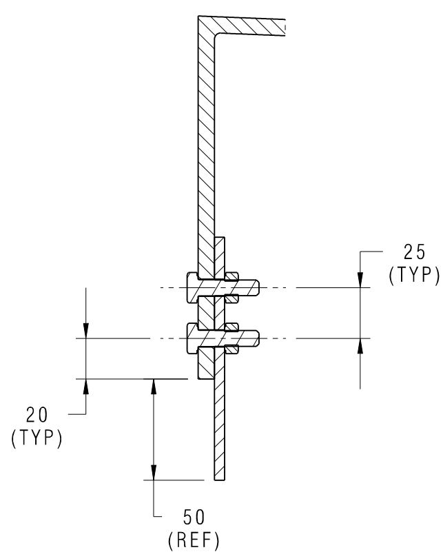
SECTION-CC SCALE: 2:5
