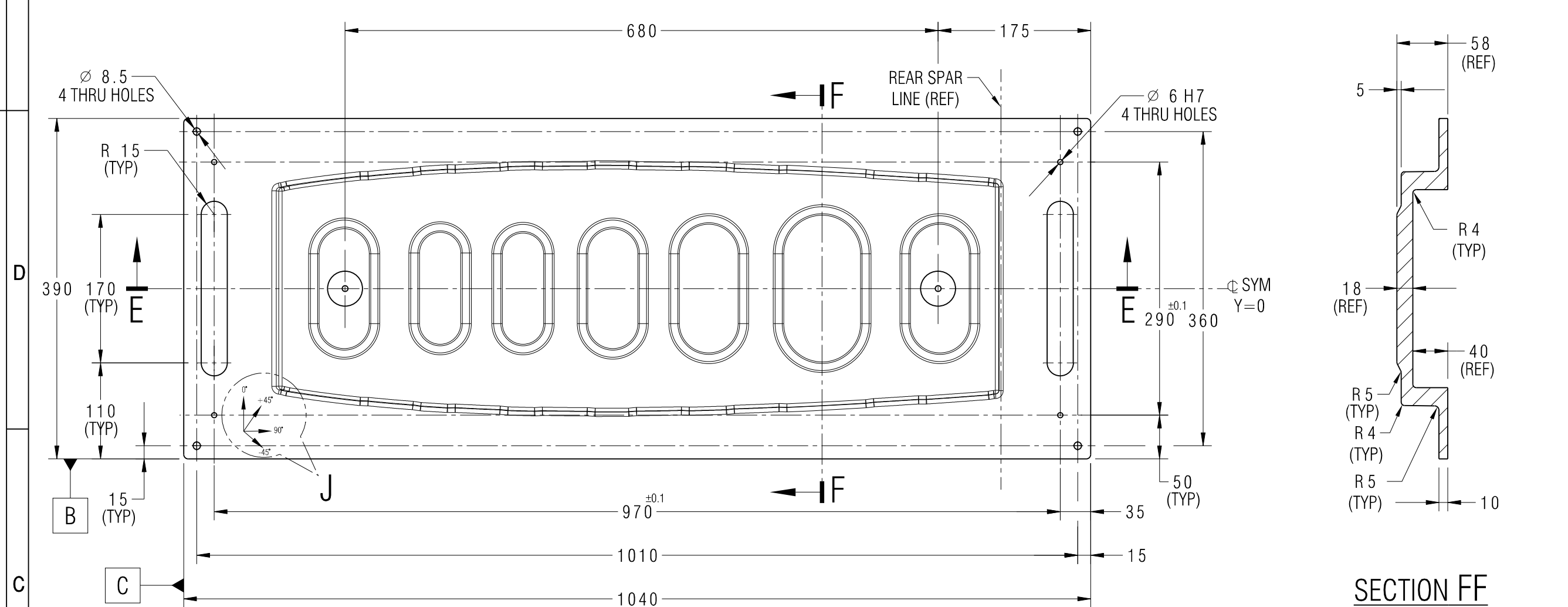
DETAIL OF ITEM No.1 (CAUL PLATE MASTER)
