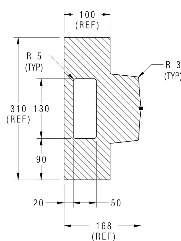
SECTION-BB
