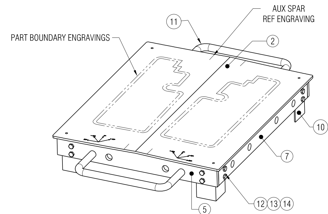
ISOMETRIC VIEW SCALE: NTS
