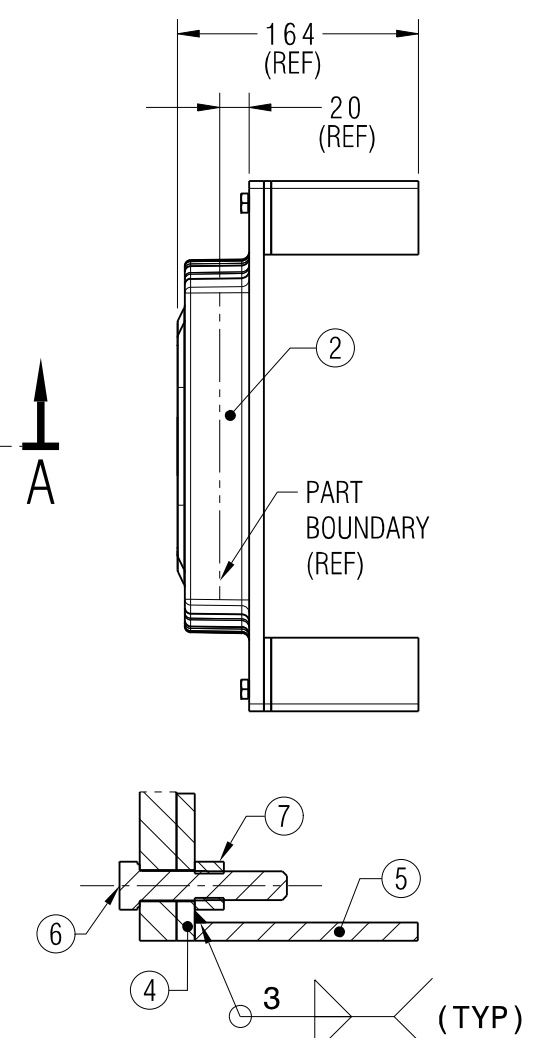
SECTION KK
