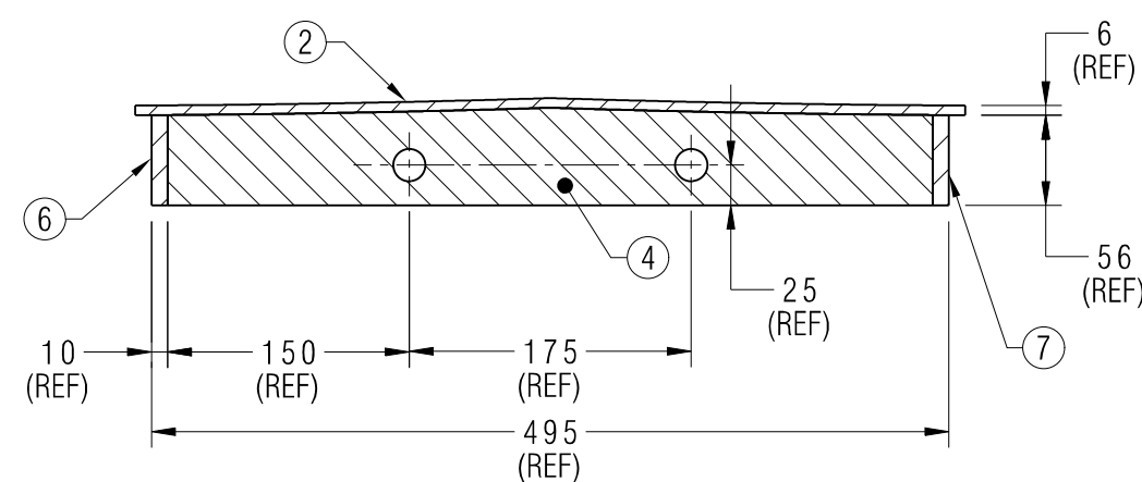
SECTION GG
