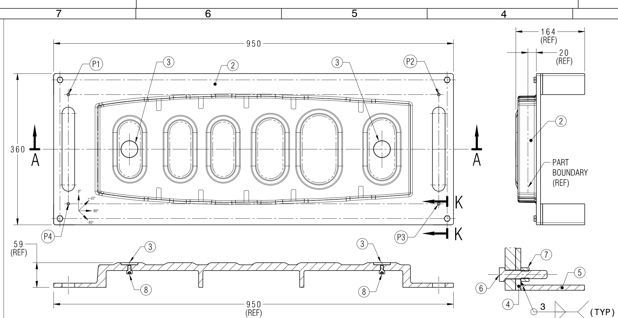
SECTION AA
