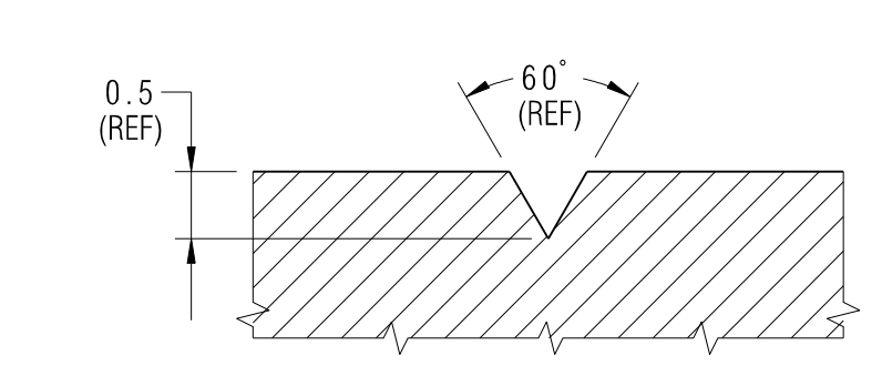
DETAIL-M (SCALE -NTS) REFER NOTE 4
