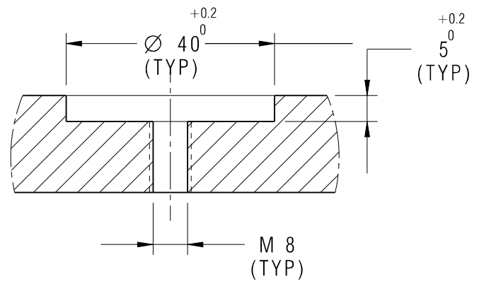
DETAIL G SIMILAR AT DETAIL H SCALE: 1:1
