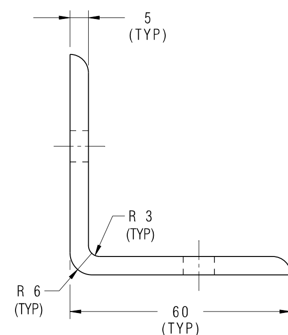
DETAIL OF ITEM NO.3 SCALE: 1:1
