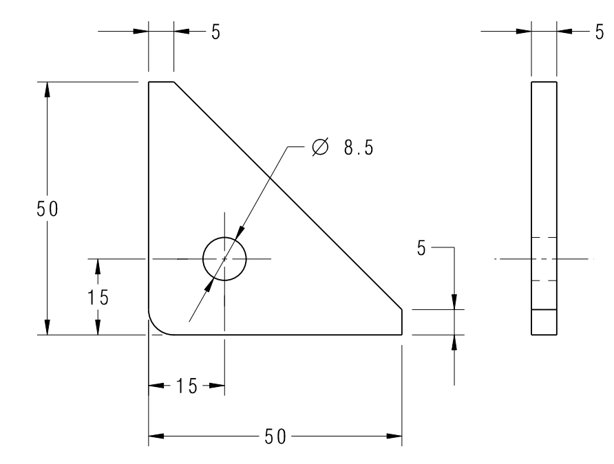
DETAIL OF ITEM NO:4 SCALE:1:1
