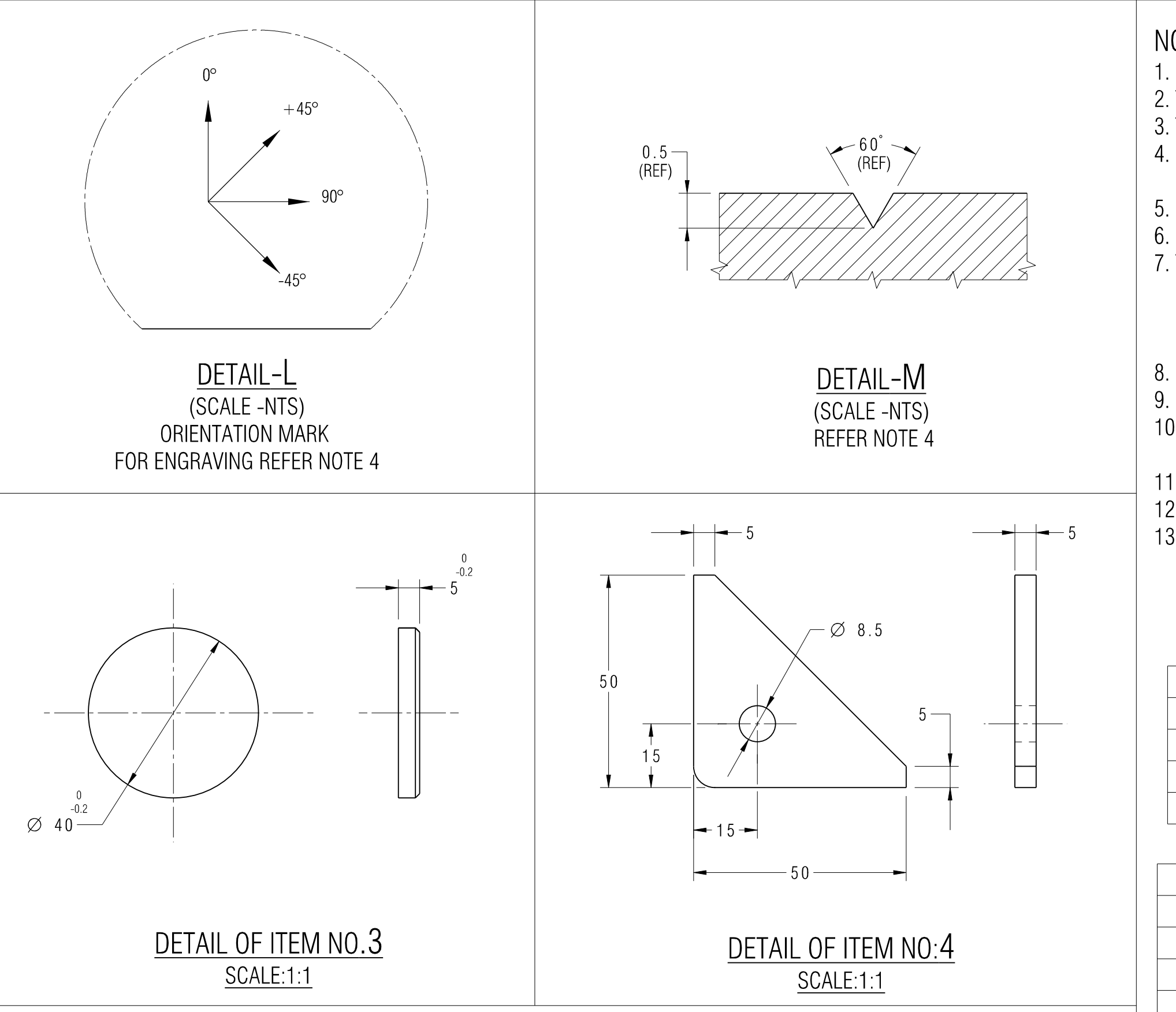
ASSEMBLY DETAILS (LAYUP CORE)
