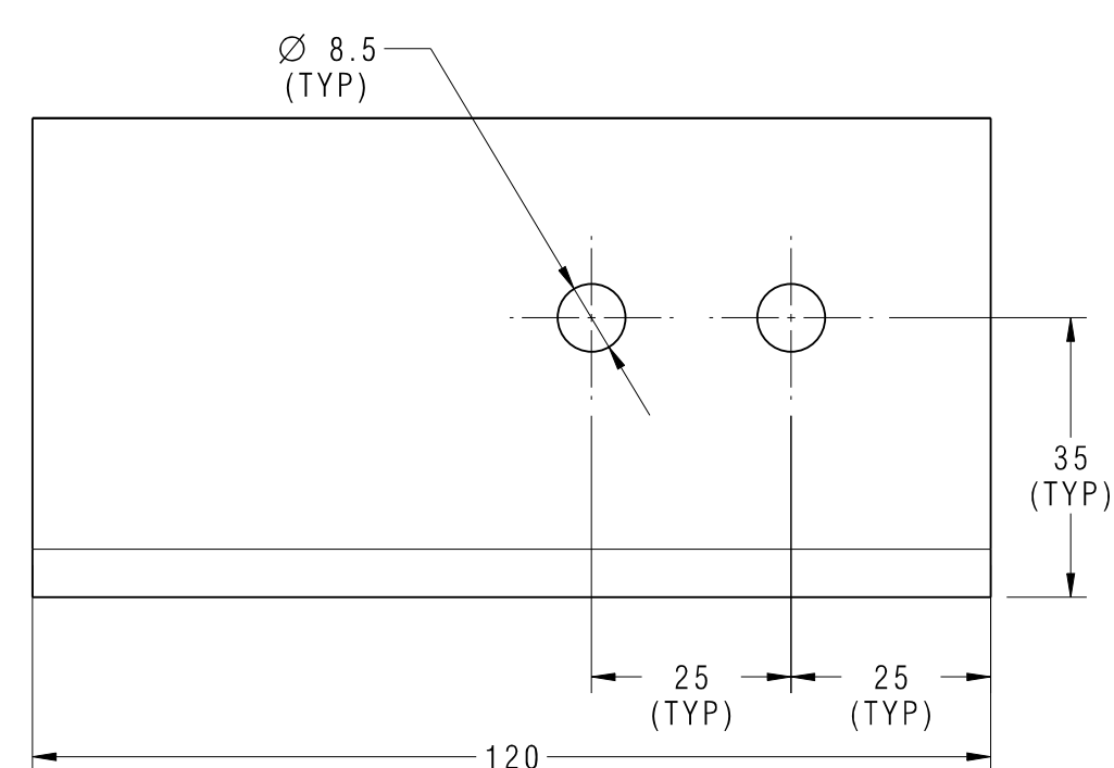
DETAIL OF ITEM NO.3 SCALE: 1:1
