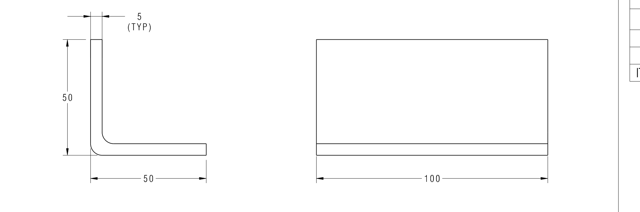
DETAIL OF ITEM NO:5 SCALE:1:1
