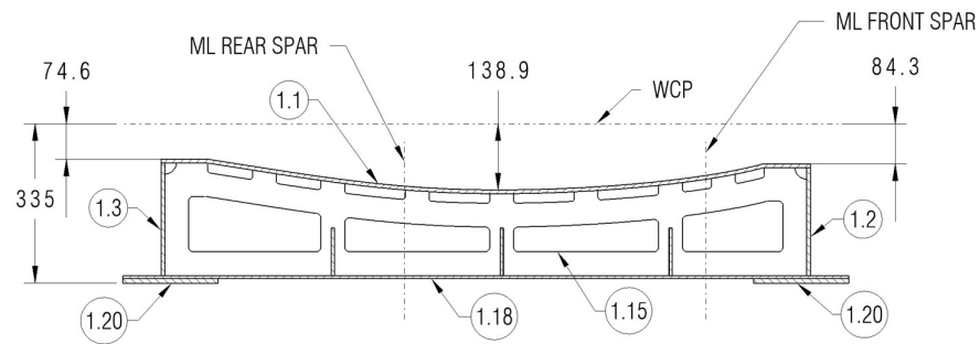
Figure 3: Typical sectional view showing transverse contour profile
