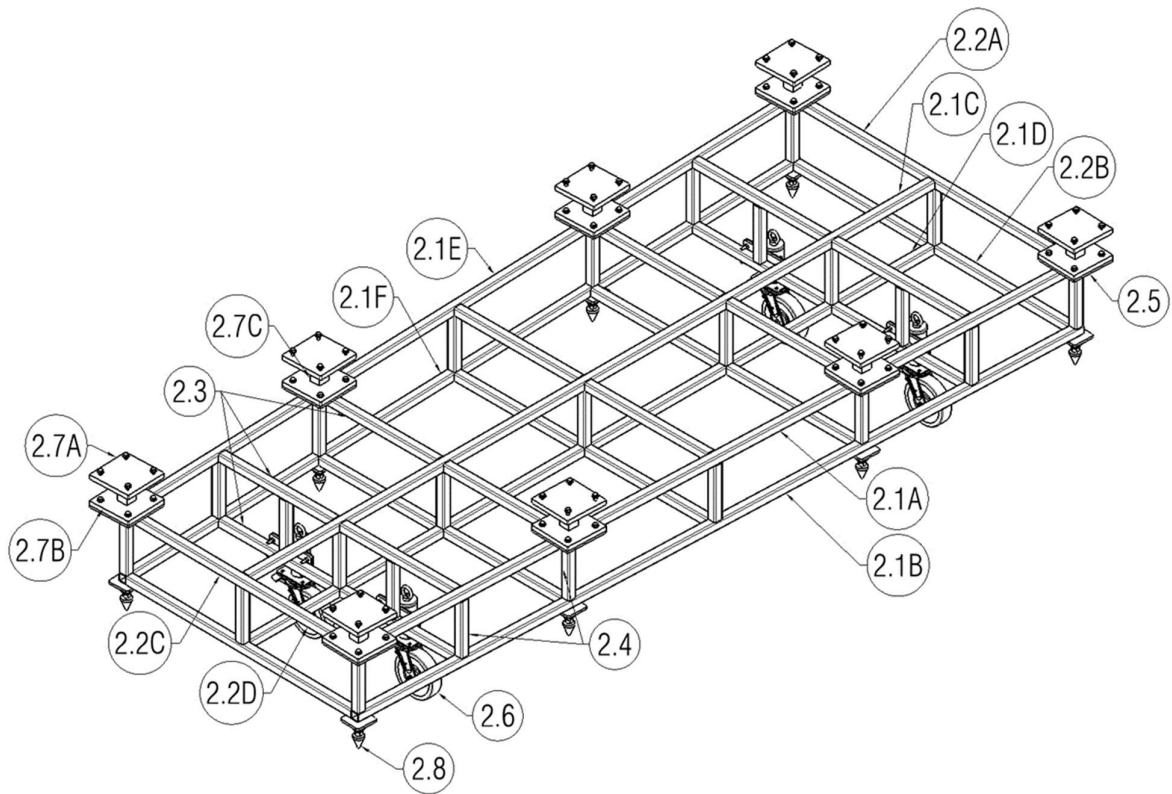
Figure 6: Wing top skin O/B LH tool support structure/trolley mechanism
