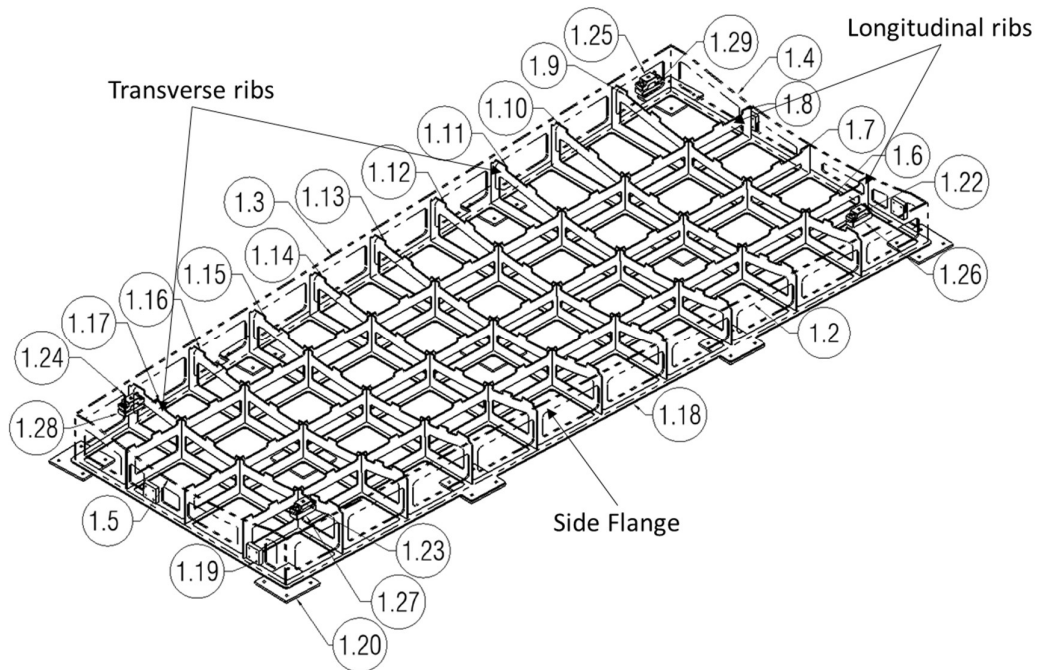
Figure 5: Wing top skin O/B LH tool backup structure (longitudinal, transverse ribs and side flanges)
