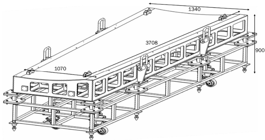
Figure 7: Wing bottom skin O/B LH tool including backup structure and support structure
