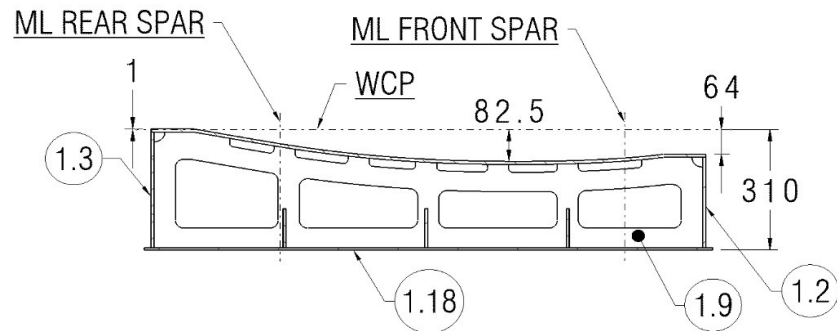
Figure 8: Typical sectional view showing longitudinal contour profile
