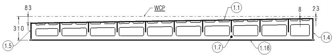
Figure 8: Typical sectional view showing longitudinal contour profile
