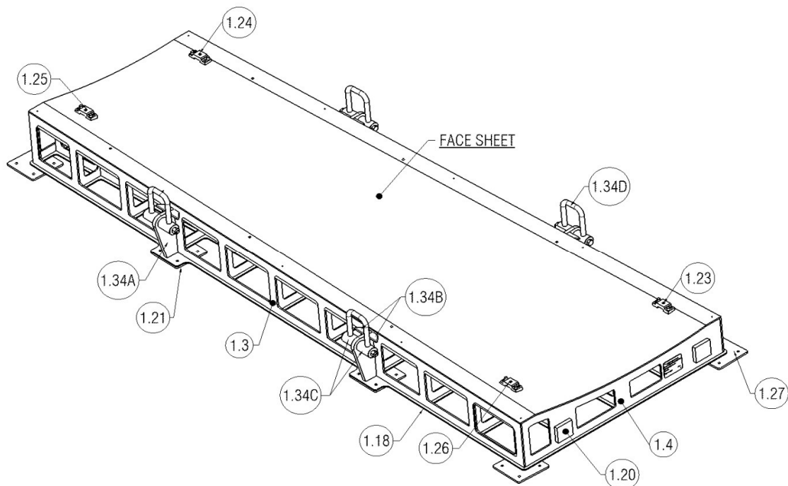
Figure 10: Wing bottom skin O/B LH tool, face sheet with backup structure
