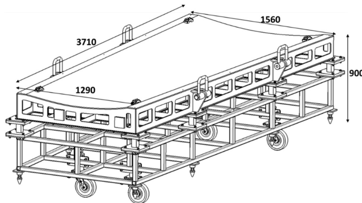
Figure 1: Wing top skin O/B LH tool including backup structure and support structure
