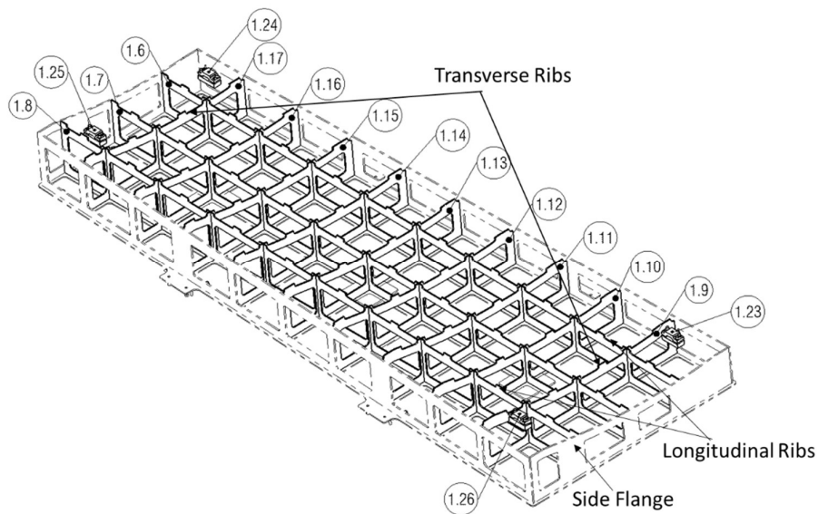
Figure 11: Wing bottom skin O/B LH tool backup structure (longitudinal, transverse ribs and side flanges)
