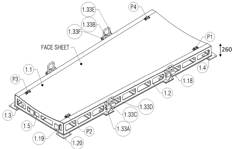
Figure 4: Wing top skin O/B LH tool, face sheet with backup structure
