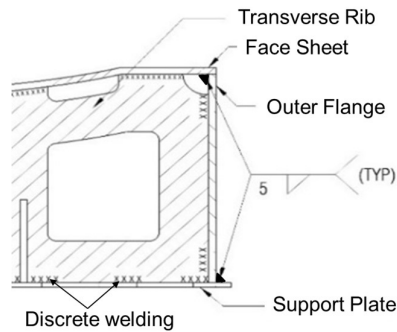
Figure 13: Typical Welding Scheme
