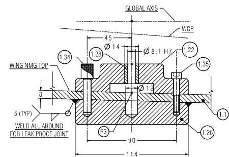
Sectional Details (all dimensions are in 'mm')
