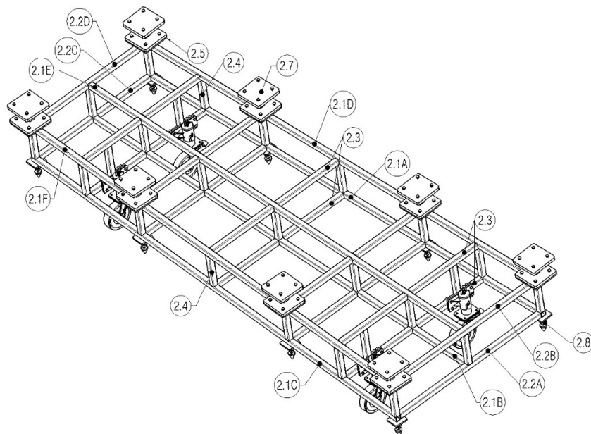
Figure 12: Wing bottom skin O/B LH tool support structure/trolley mechanism
