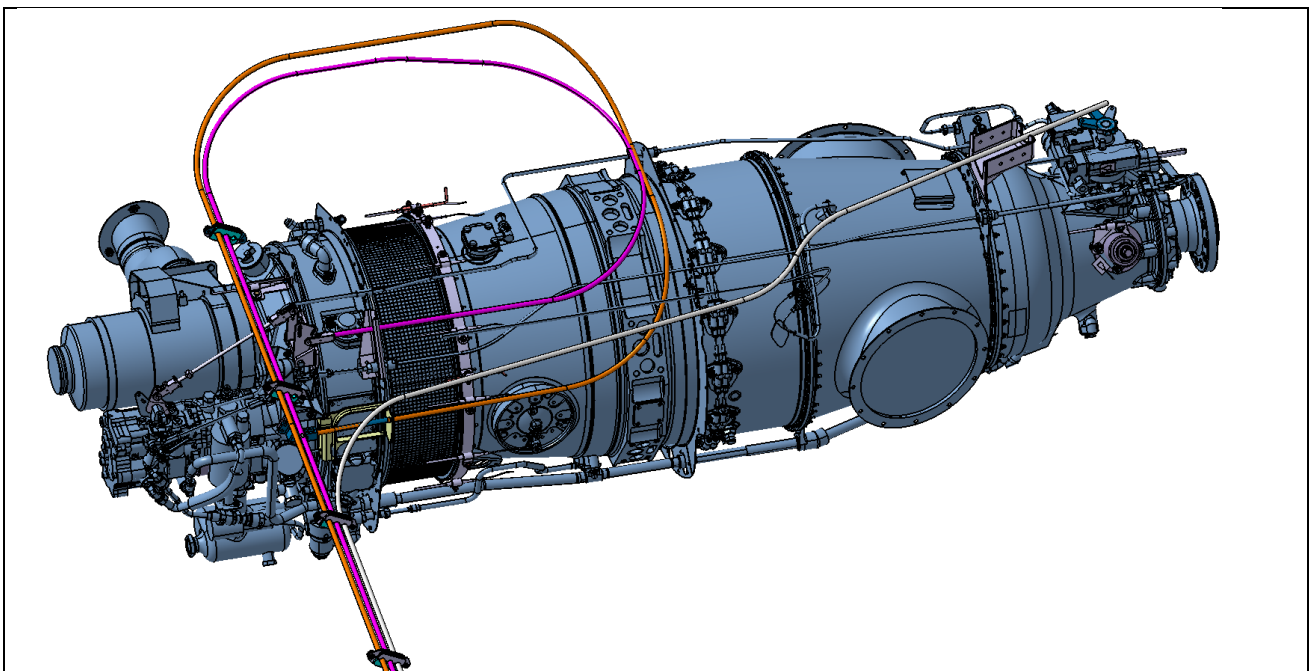
Figure 7 Routing of engine control cable in the engine nacelle for the LH engine. Orange cable: Power control cable, Purple cable: Fuel control cable, Grey cable: Propeller control cable
