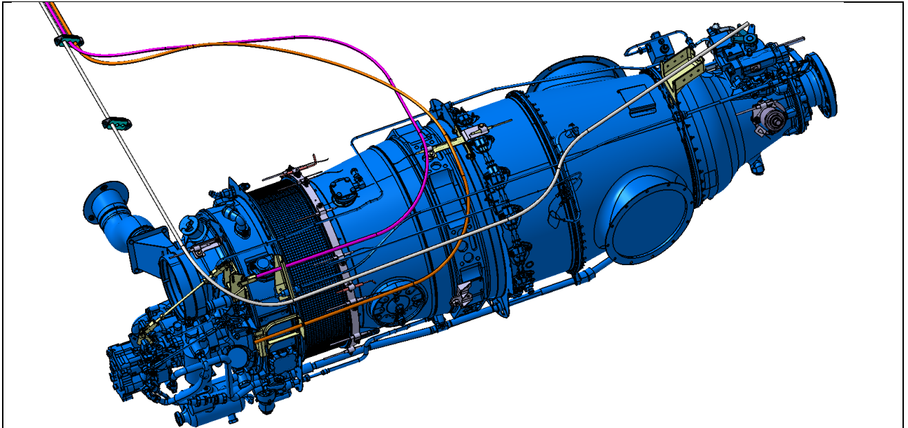
Figure 6 Routing of engine control cable in the engine nacelle for the RH engine. Orange cable: Power control cable, Purple cable: Fuel control cable, Grey cable: Propeller control cable
