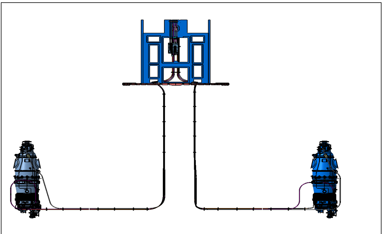
Figure 5 Top view of the layout of engine control cables from TQB to the LH and RH engines
