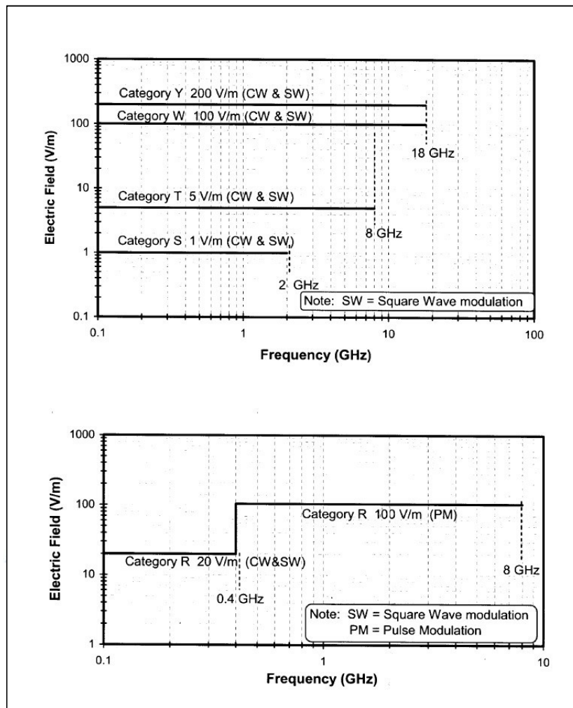
Figure 20-10 (A&B) Radiated Susceptibility Test Level
