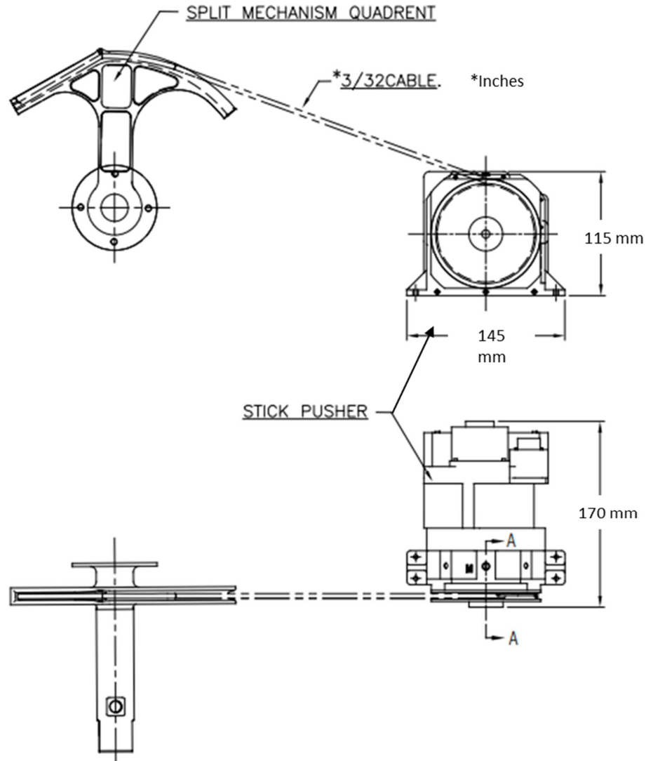
Figure 2 Stick Pusher schematic
