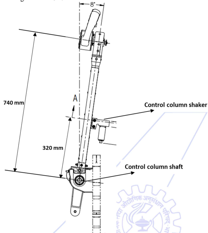
Figure 1 Schematic of control column geometry
