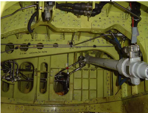
Hydraulic installation in MLG bay
